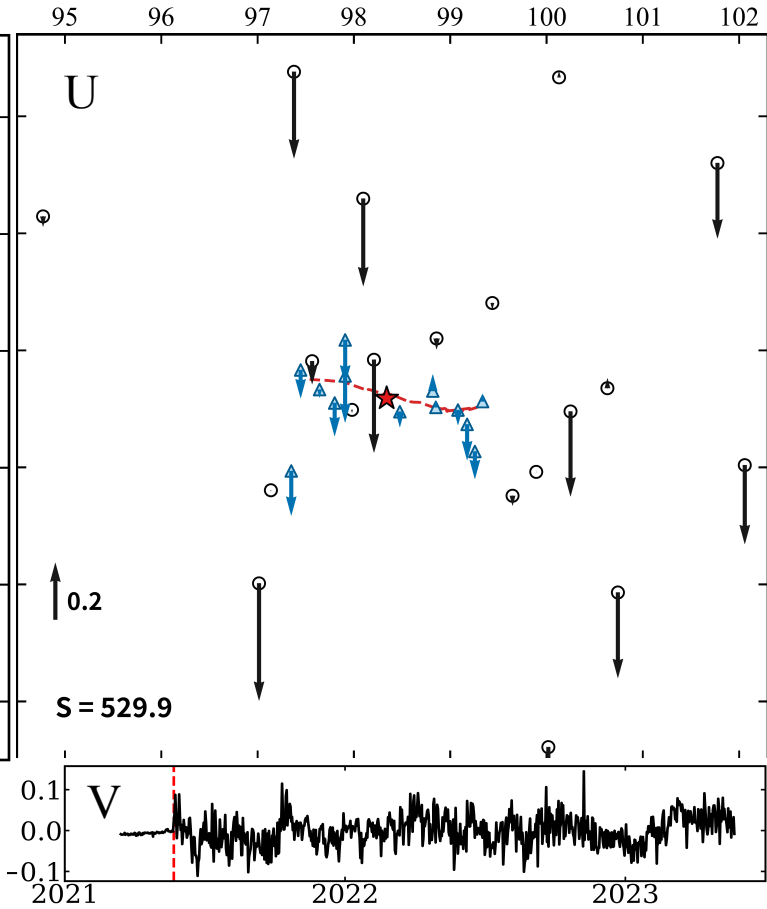
(b) Second IC
