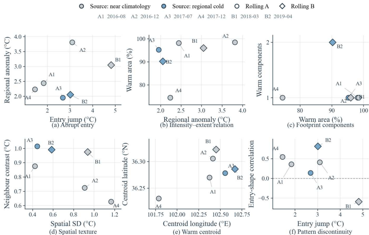
Figure 7. Entry and spatial fingerprints of six widespread-warm validation target months. Matched scatter panels encode entry jump, warm extent, footprint structure, texture, centroid, and pattern continuity.
