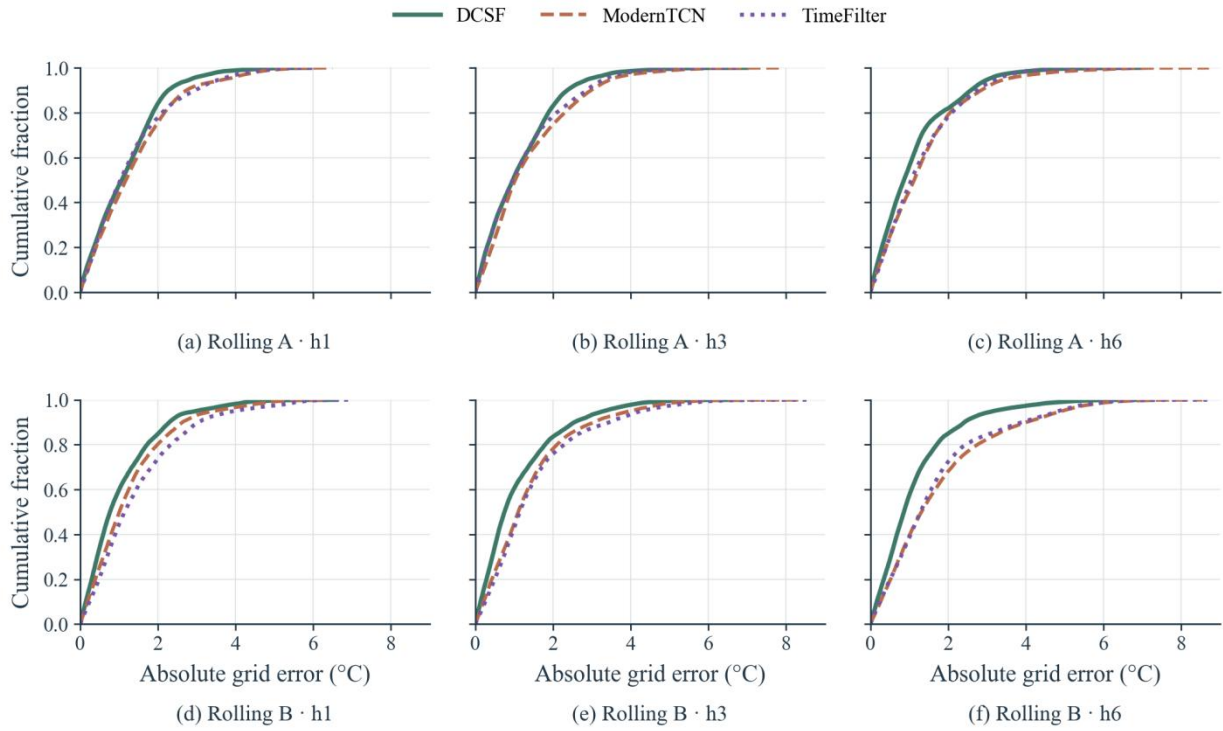
Figure 4. Complete absolute grid-error distributions across folds and forecast horizons. ECDFs compare DCSF, ModernTCN, and TimeFilter through the full ERA5-Land target-error tail.
