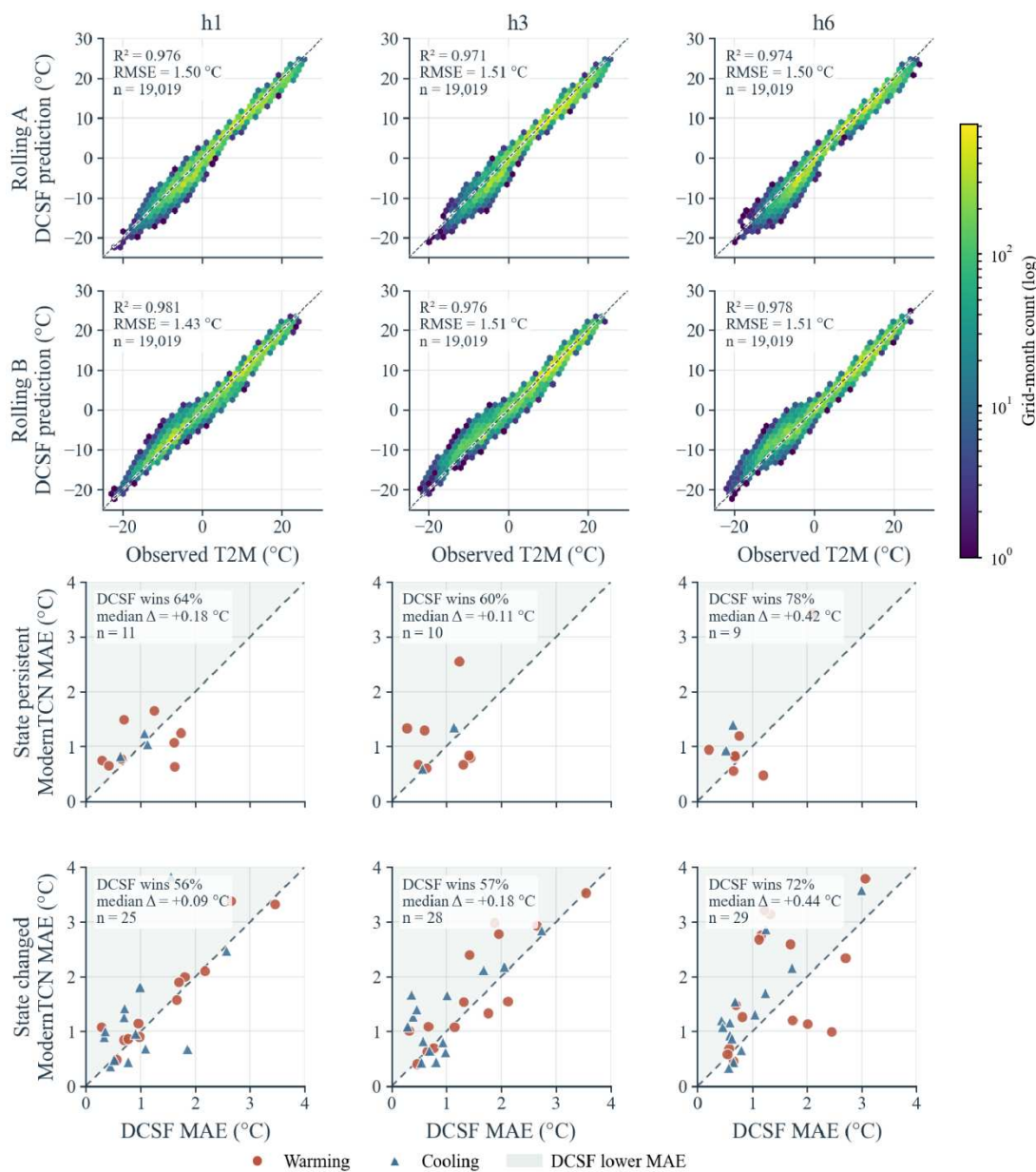
Figure 3. Absolute DCSF agreement and paired gains over ModernTCN across horizons and thermal-state conditions. Columns are h1, h3, and h6; rows show fold-wise predicted-versus-target ERA5-Land T2M and persistent/changing target-month MAE pairs.
