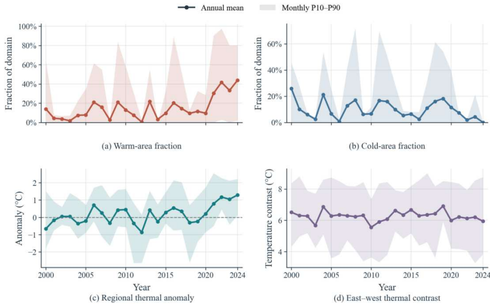
Figure 6. Evolution of ERA5-Land regional thermal structure from 2000 to 2024. Annual means and monthly P10–P90 intervals show warm and cold footprints, regional anomaly, and east–west contrast.
