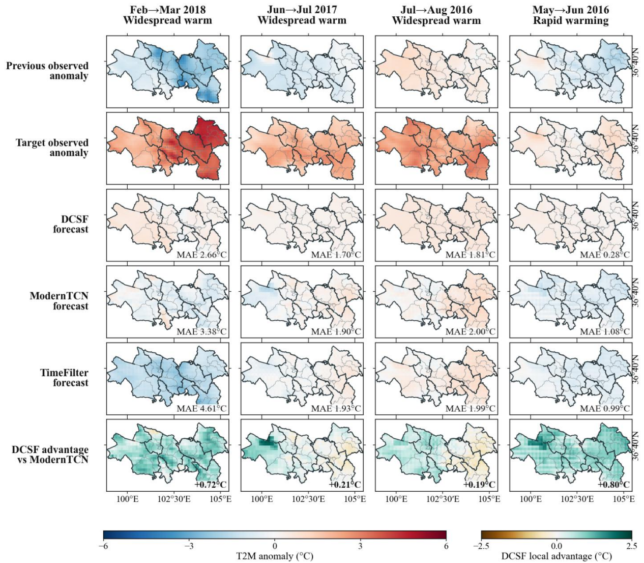
Figure 11. Spatial realization of DCSF advantage across four h1 warming transitions. Columns show four cases; rows show preceding and target anomalies, three forecasts, and local ModernTCN-minus-DCSF error gain.
