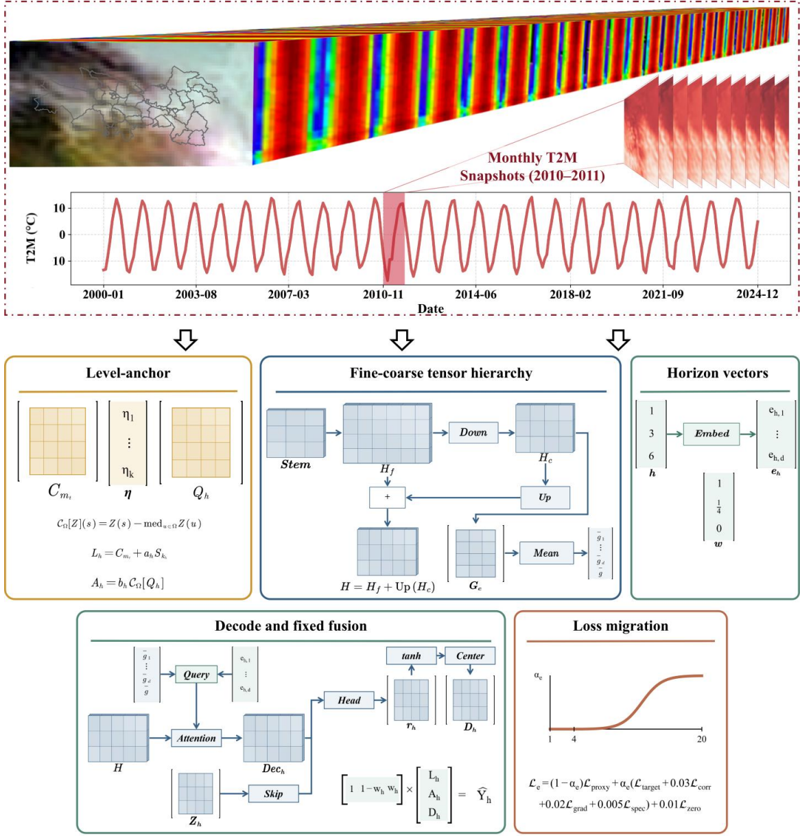
184 Figure 2. RegimeTransfer-DCSF architecture and training schedule. Panels show anchoring, tensor 185 decoding, fusion, and loss migration.
