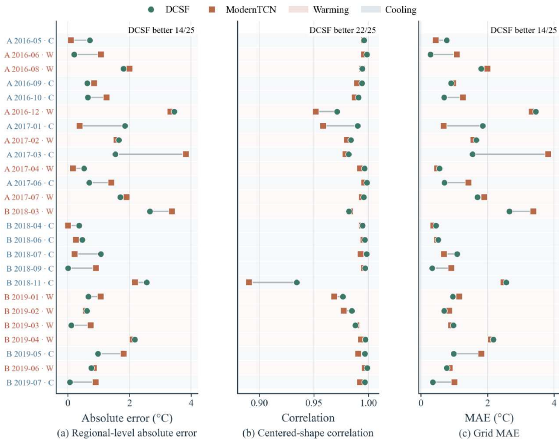
435 Figure 5. Regional-level, centred-shape, and gridwise recovery during h1 state changes. Paired 436 dumbbells compare DCSF and ModernTCN for each changing target month; W and C denote warming 437 and cooling.
