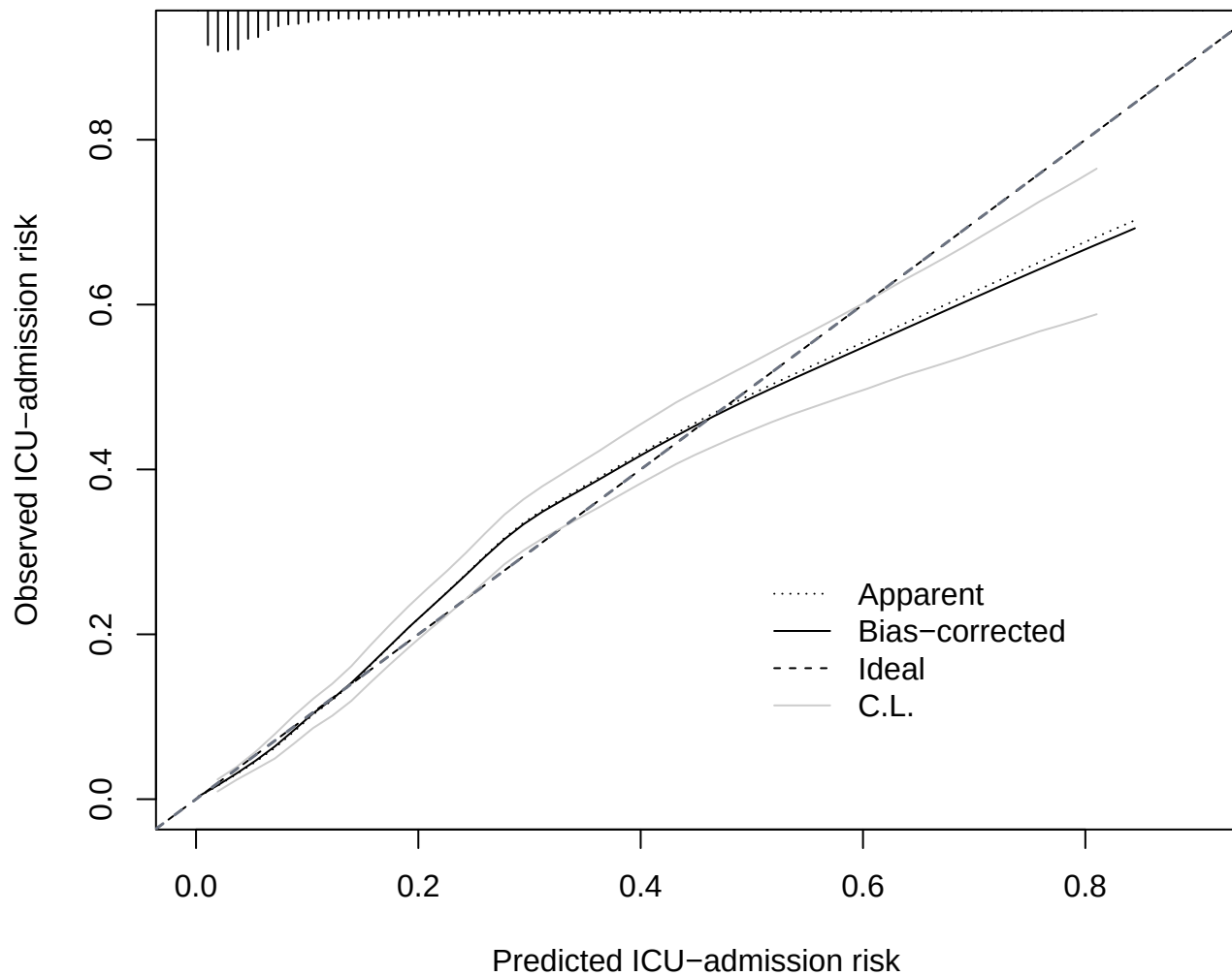
RMS bootstrap calibration curve
