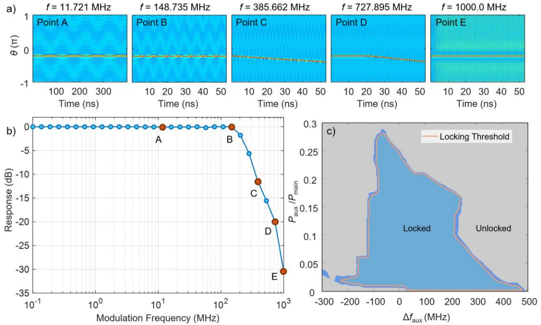
Fig. 7 | Dynamic trapping limits and locking phase diagram. (a) Time-domain soliton tracking snapshots corresponding to specific modulation frequencies (A–E) as the scanning speed approaches the dynamic threshold. (b) Tracking fidelity as a function of phase-scanning rate. A broad plateau is observed under stable locking, followed by a rapid roll-off associated with Adler unlocking and phase slipping. (c) Two-dimensional locking phase diagram as a function of auxiliary-pump frequency detuning from the DW resonance (horizontal axis) and auxiliary-to-main pump power ratio (vertical axis). The colored regions distinguish the dynamically locked and unlocked operating regimes. The boundary indicates the locking threshold, demonstrating the parameter space over which stable soliton trapping can be maintained.
