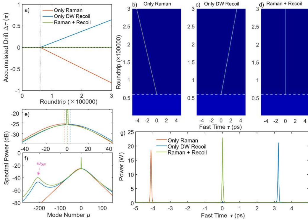
Fig. 4 | Raman self-frequency shift compensation via engineered DW recoil. (a) Temporal drift trajectories of single solitons simulated from identical initial noise seeds. The red and blue curves correspond to the Raman-only and DW-only cases, respectively, while the green curve tracks the stationary force-balanced state. (b)-(d) Long-term temporal evolution maps for the (b) Raman-only, (c) DW-only, and (d) Force-balanced states, respectively. (e) High-resolution spectral view around the pump resonance, with dashed lines indicating the calculated spectral CoM positions. (f) Corresponding full optical spectra and (g) Temporal pulse profiles for the three operating conditions.
