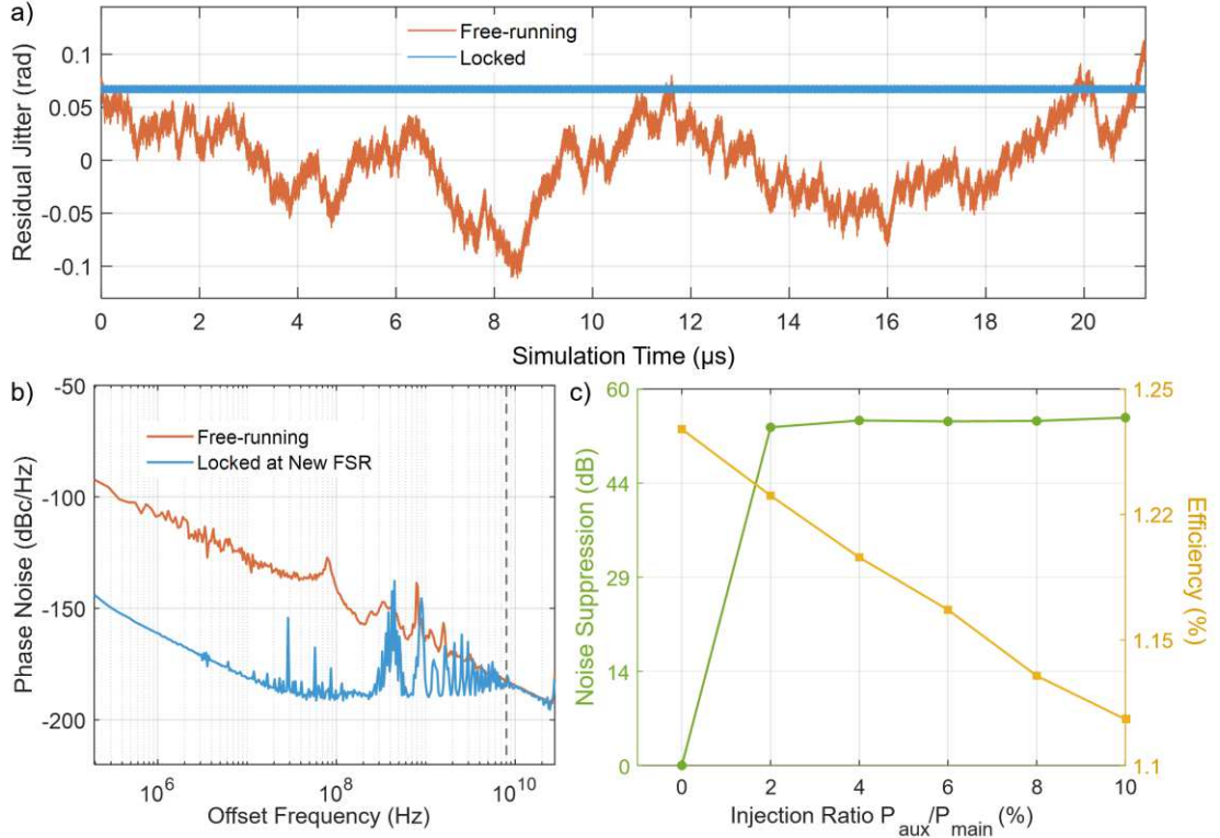
Fig. 8 | Simulated noise suppression and timing stabilization via active DW locking. (a) Residual phase jitter of the free-running and locked states. The free-running state exhibits large random-walk fluctuations arising from unconstrained timing diffusion, whereas the locked state remains tightly confined around a stable equilibrium position. (b) Simulated single-sideband phase-noise power spectral density (PSD) of the free-running and locked states. (c) Phase-noise suppression (green, left axis) and microcomb conversion efficiency (yellow, right axis) plotted against the auxiliary-to-main injection power ratio. Significant noise reduction is achieved with auxiliary-power fractions of only a few percent, while the comb conversion efficiency remains nearly unchanged.
