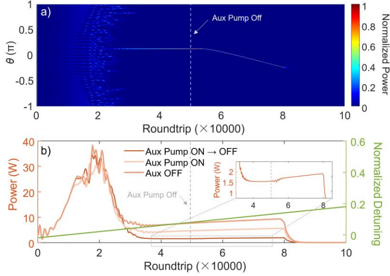
Fig. 5 | Active trapping and preservation of soliton existence. (a) Simulated time-domain evolution illustrating the temporal trapping of a dissipative Kerr soliton. The soliton trajectory remains tightly localized during the application of the auxiliary pump and progressively reverts to a free-running random-walk regime after the auxiliary field is removed (indicated by the dashed line). (b) Intracavity energy evolution for three operating conditions: continuous auxiliary pumping, no auxiliary pumping, and auxiliary-pump removal. The normalized pump detuning is shown on the right axis (green curve). The inset zooms in on the transient energy variations induced by switching the auxiliary pump off. The negligible perturbation confirms that temporal trapping does not significantly alter the soliton existence conditions.
