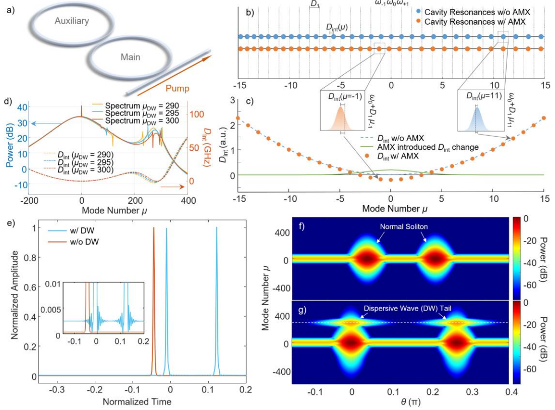
Fig. 1 | Principle of deterministic dispersion engineering and dispersive wave emission. (a) Schematic of the coupled dual-ring microresonators system. (b) Resonance frequency distribution without (blue dots) and with (orange dots) mode splitting induced by the auxiliary resonator. (c) Integrated dispersion D_{\text{int}} profiles showing the unperturbed parabolic dispersion (blue dashed line), the perturbed dispersion (red symbols), and the localized dispersion modification induced by the AMX (green curve, representing the difference between the perturbed and unperturbed states). (d) Simulated soliton spectra and corresponding D_{\text{int}} profiles under varying coupling conditions. (e) Temporal waveforms of an unperturbed soliton (orange curve) and a DW-engineered soliton (blue curve); the inset shows a magnified view of the trailing oscillatory tail. (f, g) Time-frequency spectrograms of (f) an unperturbed soliton and (g) DW-engineered soliton, demonstrating that the temporal oscillations originate from localized radiation at the phase-matched mode index \mu_{\text{DW}} .
