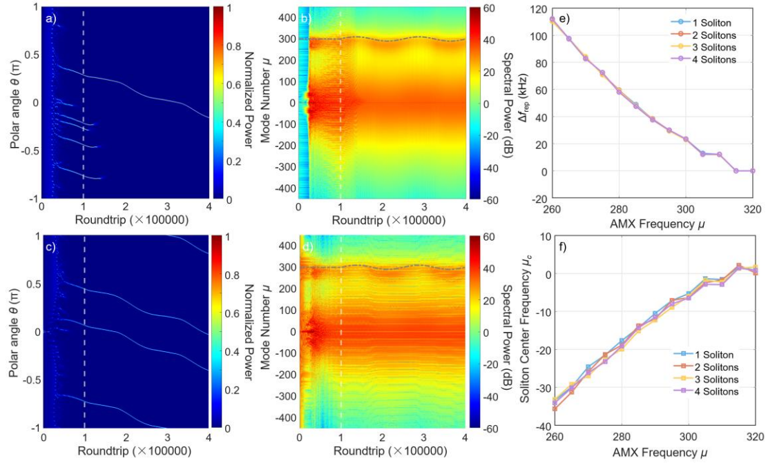
Fig. 2 | Kinematic control via DW emission. (a) Time-domain, and (b) frequency-domain evolution profiles of a single-soliton state. Dynamically shifting the AMX frequency (gray dashed line in b) modulates the DW position, inducing a controllable tilt in the temporal soliton trajectory (a), demonstrating deterministic FSR manipulation. (c) Time-domain, and (d) frequency-domain evolution for a four-soliton state. Similar spectral tracking and temporal drift dynamics are observed despite the different soliton numbers. (e) Repetition-rate shift \Delta f_{\text{rep}} and (f) Spectral center-of-mass shift as functions of the AMX position for one-, two-, three-, and four-soliton states. The overlapping tuning curves indicate that the recoil-induced repetition-rate control is independent of the number and arrangement of solitons within the cavity.
