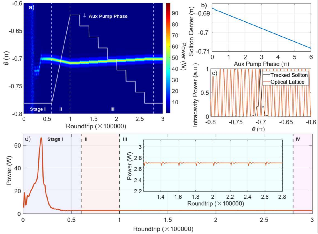
Fig. 6 | Temporal tweezing through phase-controlled optical trapping. (a) Stage I: soliton generation through primary-pump frequency sweeping. Stage II: linear scanning of the auxiliary-pump phase \phi_{aux} (solid white line), from 0 to 2\pi . Stage III: abrupt phase reset from 2\pi to 0. Stage IV: fixed auxiliary phase. (b) Relative soliton position as a function of auxiliary-pump phase, demonstrating a linear phase-to-position transduction and deterministic control of the soliton temporal coordinate. (c) Schematic illustration of temporal tweezing. The soliton remains trapped at a finite phase offset from the minimum of the phase-controlled optical potential U(\tau) formed by XPM-induced interference between the auxiliary field and the intracavity background. (d) Intracavity energy evolution continuously monitored across the successive operational stages: soliton generation via main pump frequency sweeping (light purple), linear phase scanning (pink), step-wise phase jumping (green), and static phase holding (rose). The negligible energy fluctuation proves that the temporal tweezing primarily affects the soliton position while leaving the underlying soliton existence conditions essentially unchanged.
