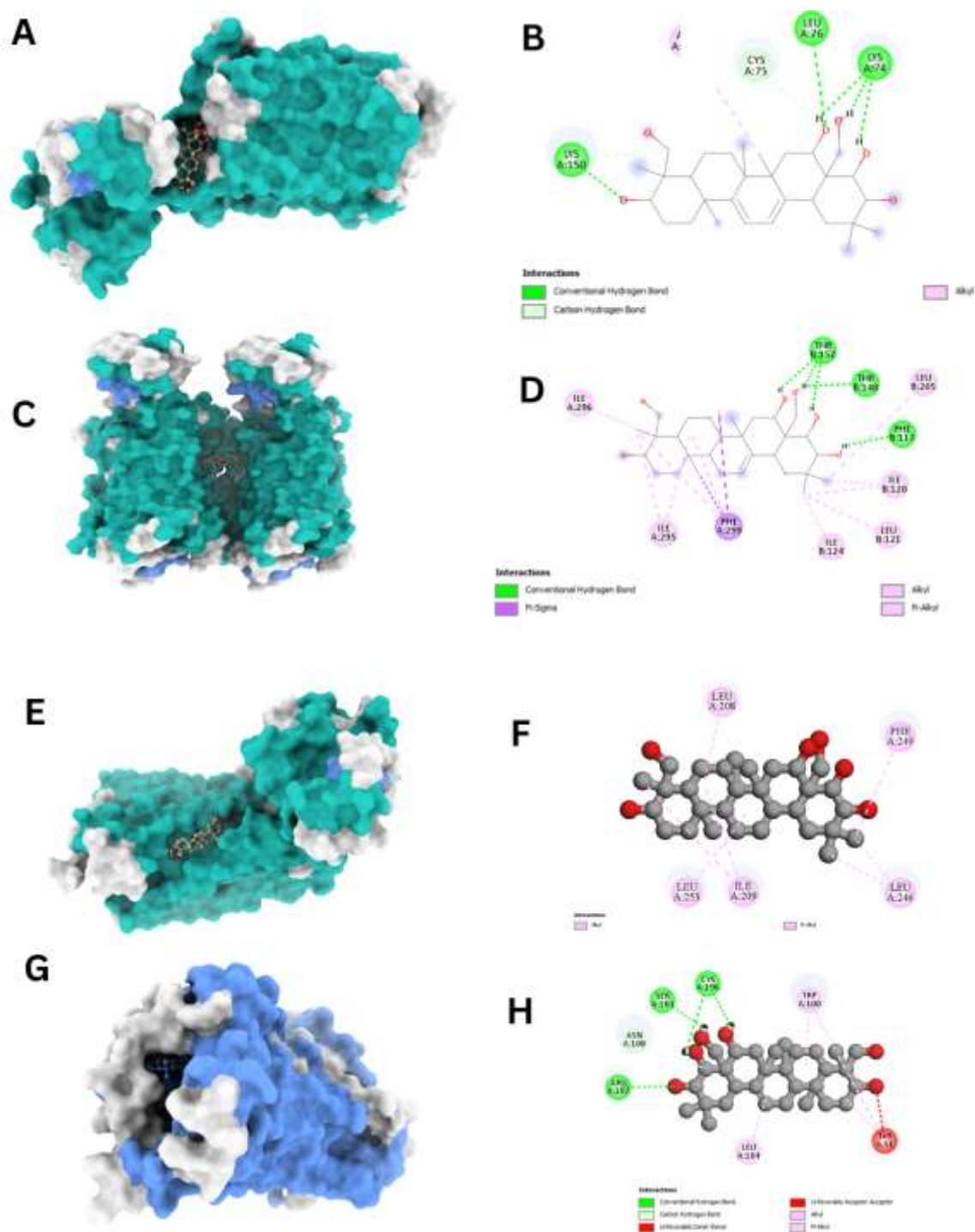
Fig. 1. Illustration of protein and ligand complex, with the left side depicting three-dimensional interactions and right side depicting two-dimensional interactions between protein and ligand (A-B) Gymnemagenin-CCR2. (C-D) Gymnemagenin-CCR5. (E-F) Gymnemagenin-CXCR4. (G-H) Gymnemagenin-CXCR7.
