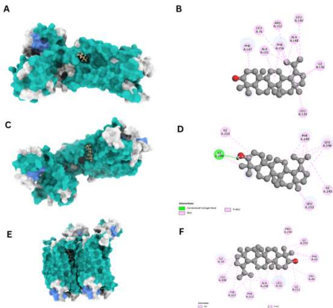
Fig. 2. Illustration of protein and ligand complex, with the left side depicting three-dimensional interactions and right side depicting two-dimensional interactions between protein and ligand (A-B) Lupeol-CCR2. (C-D) Lupeol-CXCR4 (E-F) Lupeol-CCR5
