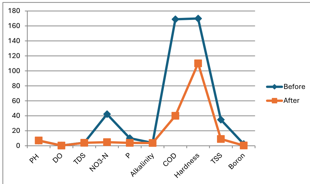
Figure 7: Line chart of wastewater physicochemical parameters at the waterlogged drainage line (flowing) before and after filtration.
