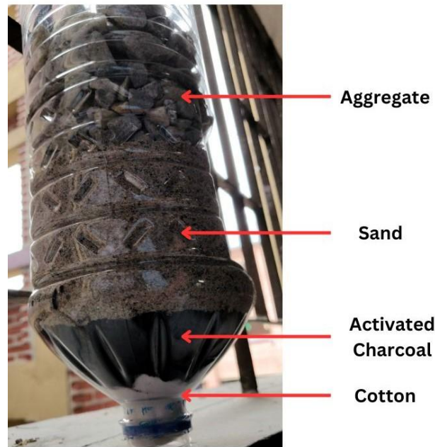
Figure 6: Visual representation of the filter sample utilized during wastewater treatment
