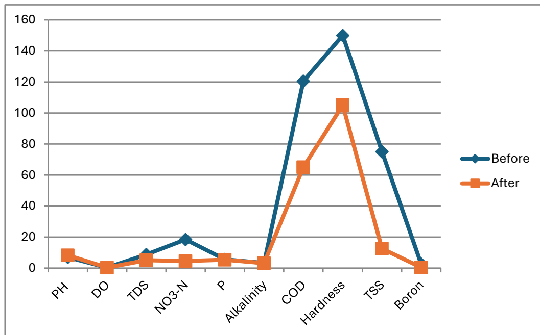
Figure 9: Line chart of wastewater physicochemical parameters at the drainage line of the central pond (flowing) before and after filtration.
