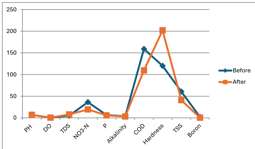
Figure 8: Line chart of wastewater physicochemical parameters at the waterlogged area (stagnant) before and after filtration.
