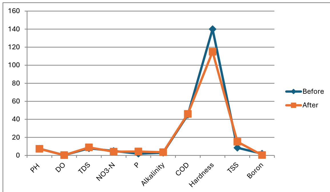
Figure 10: Line chart of wastewater physicochemical parameters at the central pond (stagnant) before and after filtration.
