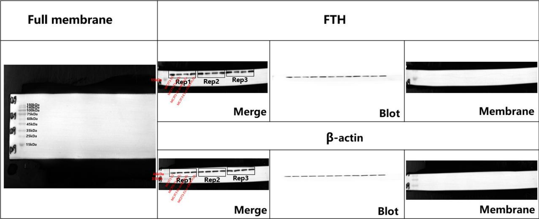
Figure 4I ALP/Runx2
