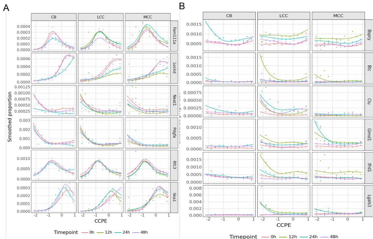
Supplementary Figure 4: novel genes show cell cycle correlation after ISC ablation. A) Plot showing normalised expression across the cell cycle for a set of core cell cycle associated genes in both homeostasis and ablation conditions. B) Plot showing normalised expression across the cell cycle for a set of genes that cell cycle associated under ablation but not homeostatic conditions.
