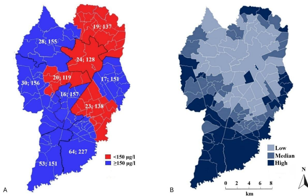
Figure 4 – Map of the city of Curitiba illustrating the distribution of the median UIC in different areas, categorized as \geq 150 \mu\text{g/l} and < 150 \mu\text{g/l} (A) and social vulnerability (risk) (B).
