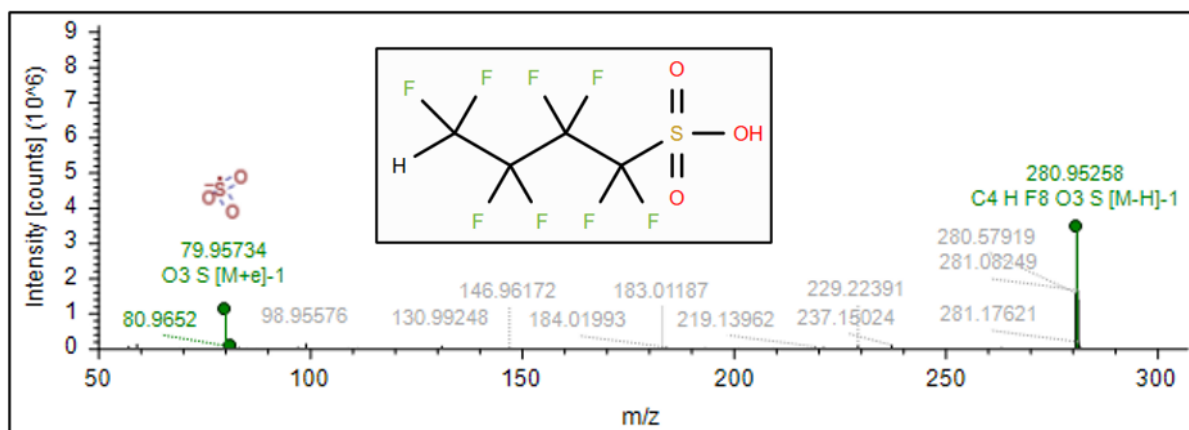
Fig. S2 Structure and MS/MS fragment ion spectrum of H-PFBS
