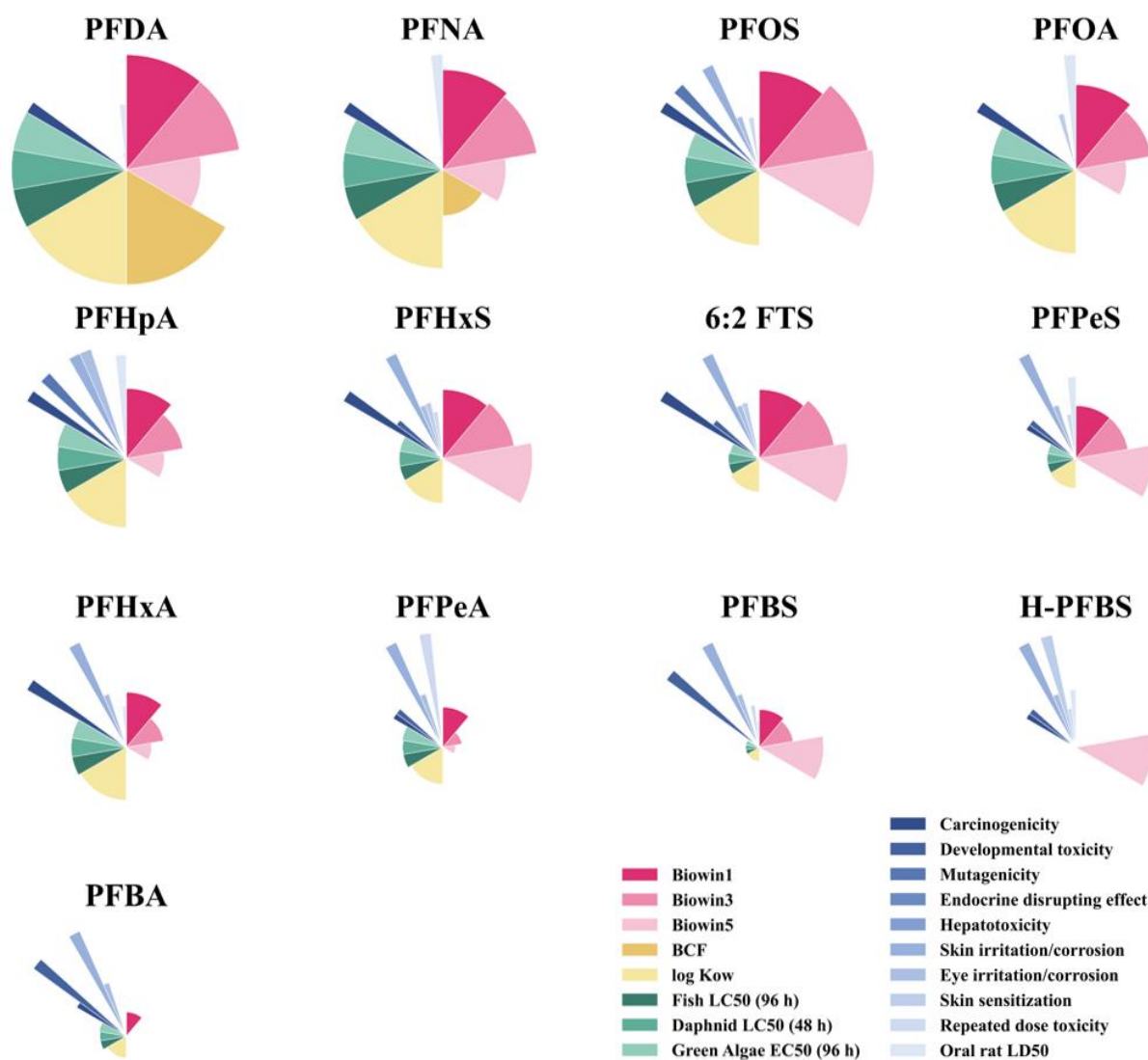
Fig. S4 Pie charts of 13 PFAS by ToxPi score
