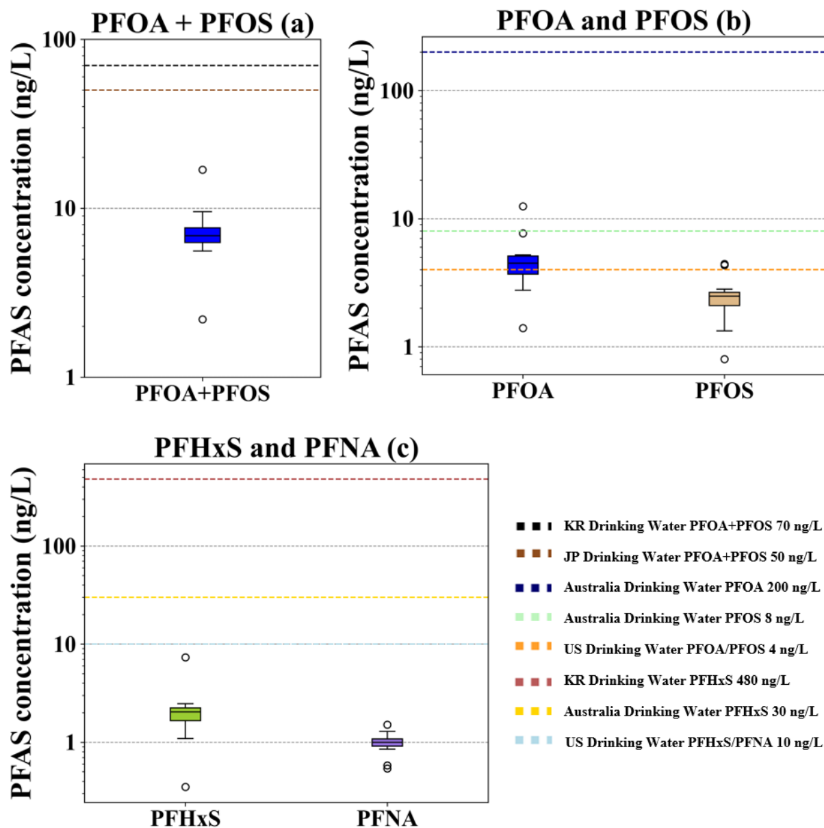
Fig. S3 Concentrations of individual PFAS in Geum River with Korea, Japan, US, Australia drinking water guidelines. (a) PFOA+PFOS, (b) PFOA, PFOS, and (c) PFHxS, PFNA
