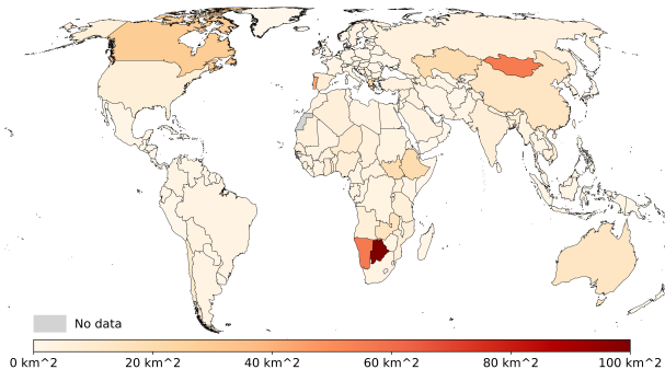
(a) Size: Mean fire size per intersection
