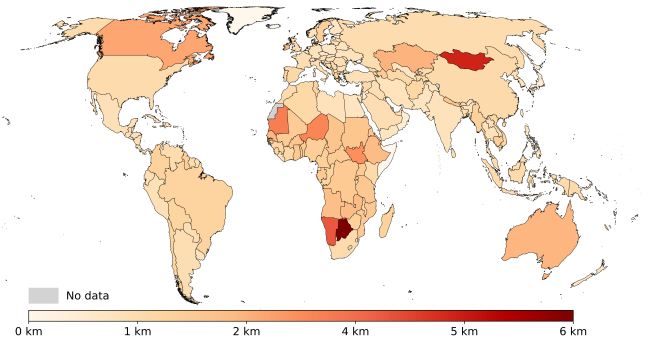
(b) Extent: Mean length of line intersected
