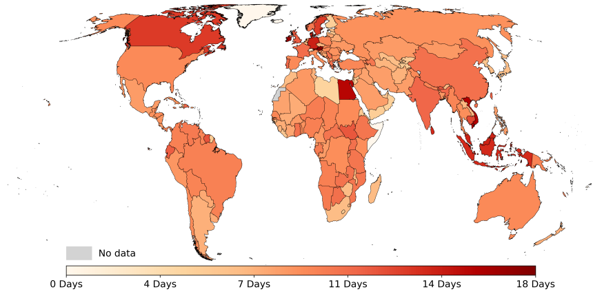
(c) Duration: Mean duration of fire per intersection
