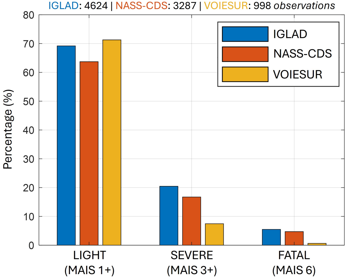
Figure 3. Vehicle-level injury severity distribution in car-to-car collisions across the IGLAD, NASS-CDS, and VOIESUR samples. Percentages represent at least light, at least severe, and fatal outcomes, determined by the maximum injury severity of the occupants for each vehicle. The share of vehicles with no injured occupants is the complement of the at least light injury distribution.
