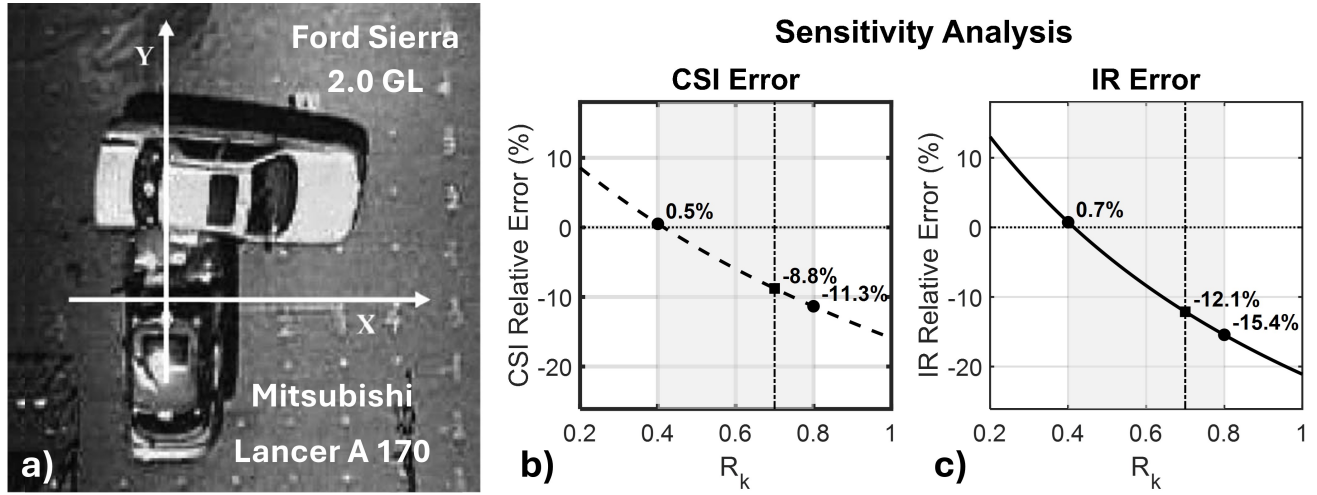
Figure 7. Initial front-to-side impact configuration of the conflicting vehicles at the point of first contact (a). Relative error propagated into the Crash Severity Index ( CSI ) prediction (b) and the corresponding at least severe injury risk ( IR_{MAIS3+} ) estimation (c) evaluated across a realistic range of the estimated vehicle stiffness ratio ( R_k ).
