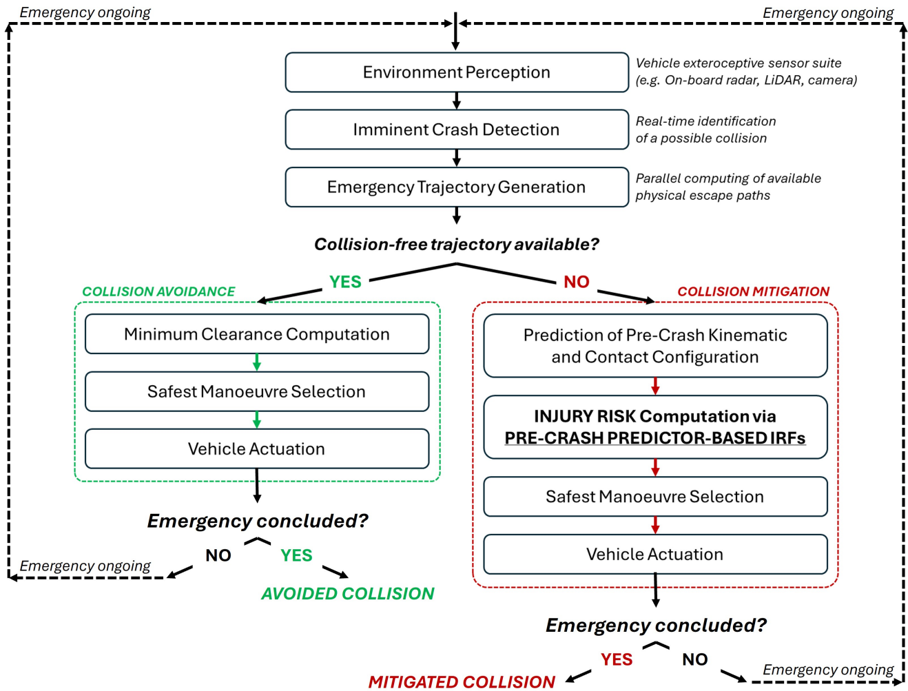
Figure 1. Functional block diagram of the proposed real-time, on-board emergency decision-making architecture.
