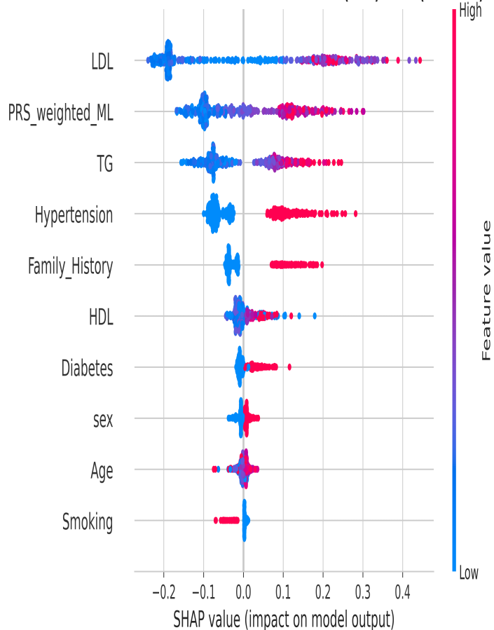
SHAP Beeswarm — RandomForest — Train (80%) — ML (with PRS)
