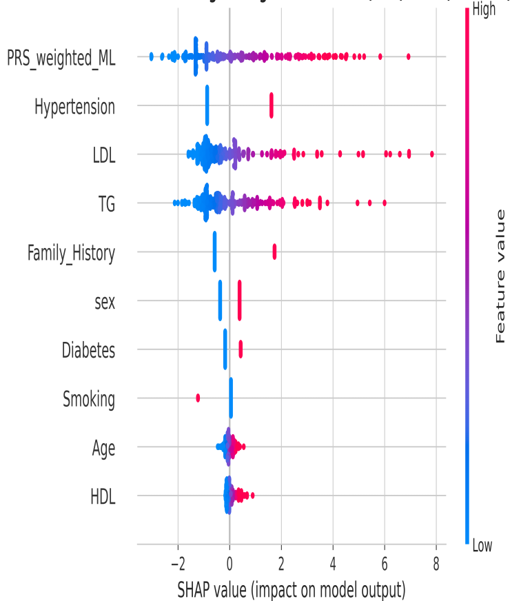
SHAP Beeswarm — LogisticRegression — Train (80%) — ML (with PRS)
