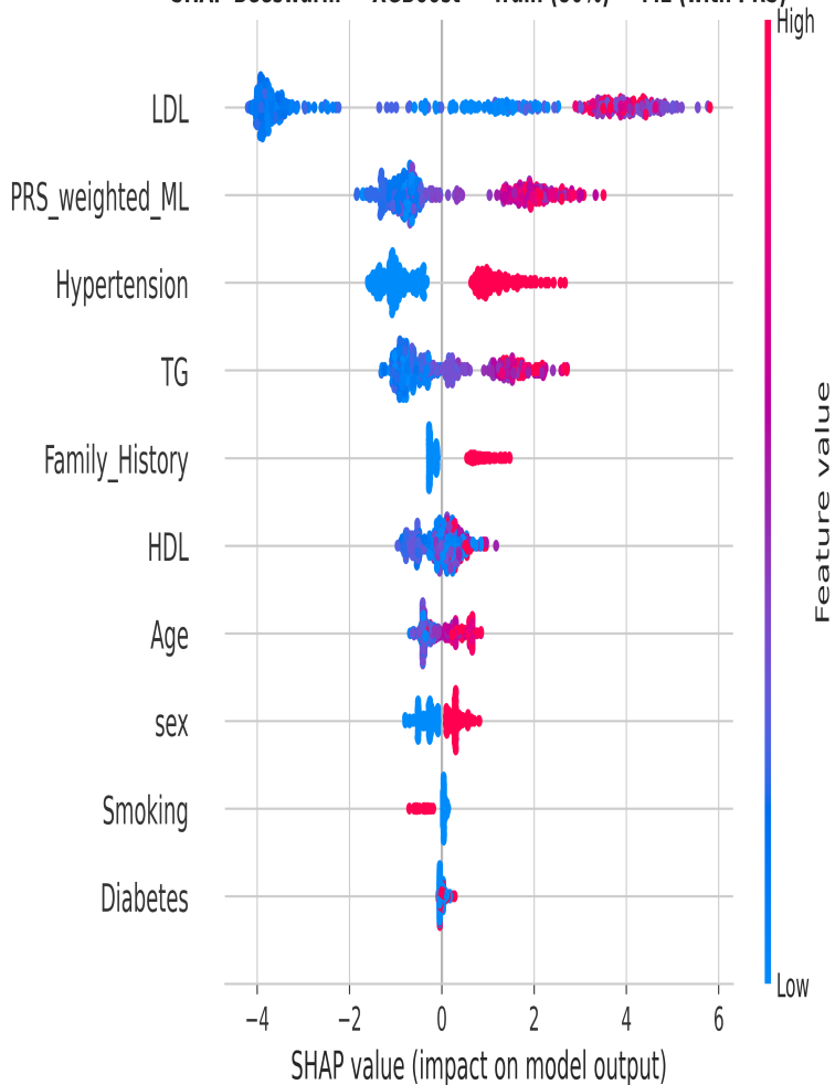
SHAP Beeswarm — XGBoost — Train (80%) — ML (with PRS)
