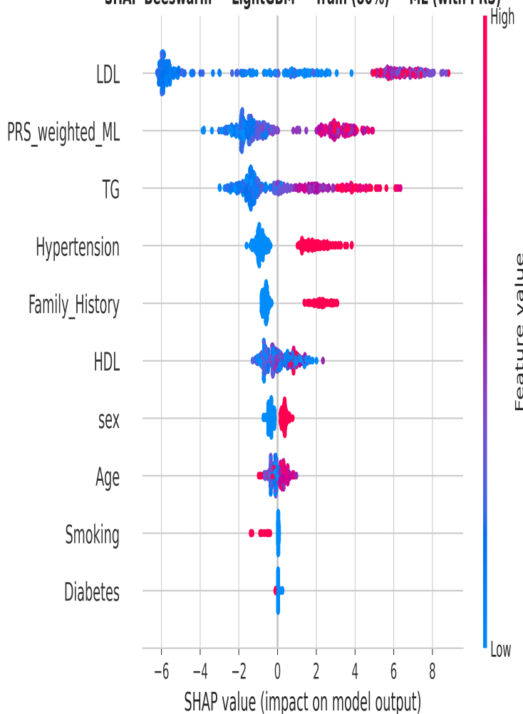
SHAP Beeswarm — LightGBM — Train (80%) — ML (with PRS)
