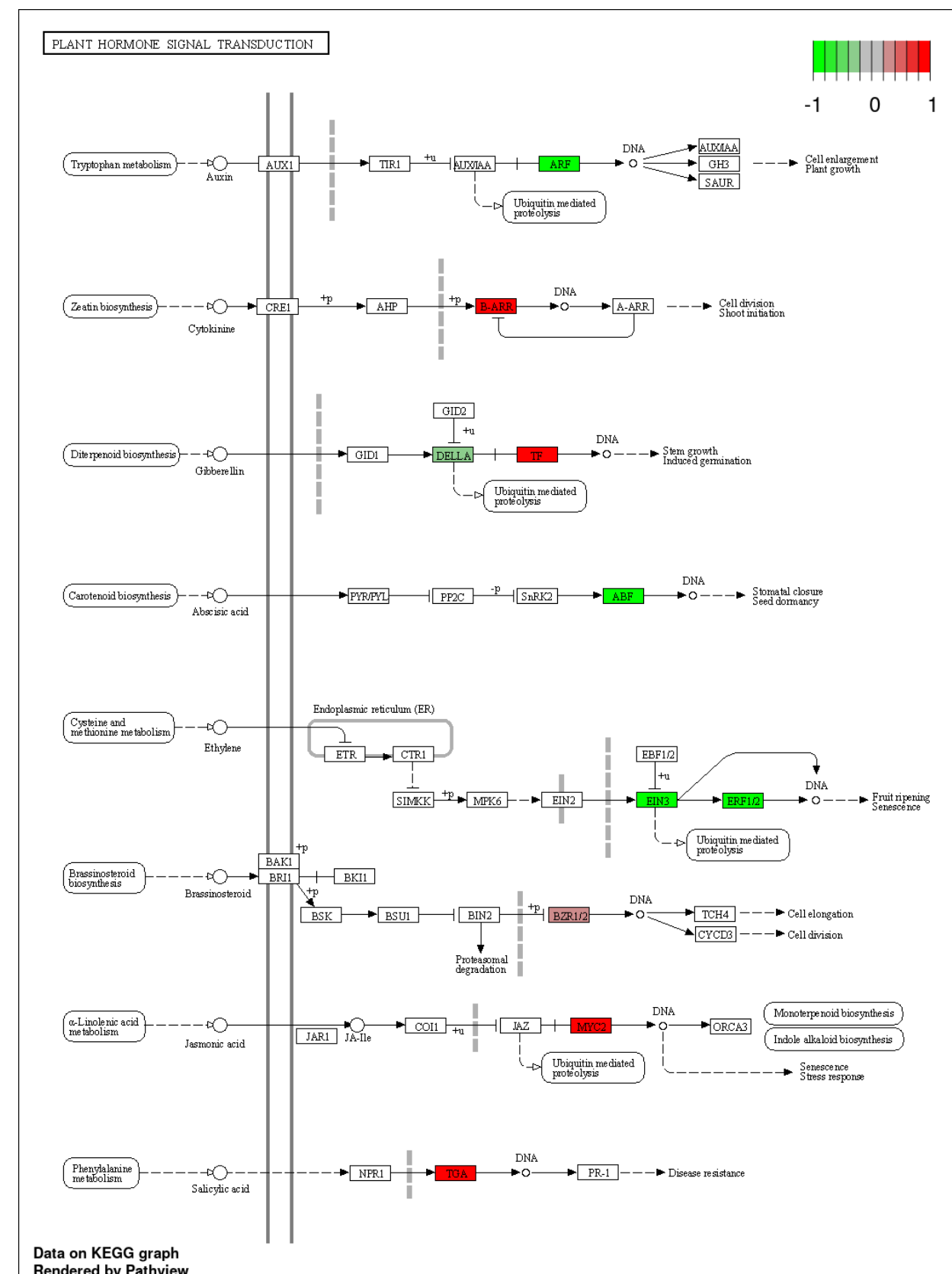
Fig. S7 KEGG graph for interaction terms cultivar x Time. On the left, 48 h.p.i; Right, 96 h.p.i. Red and green represent up- and down- regulated genes, respectively.
