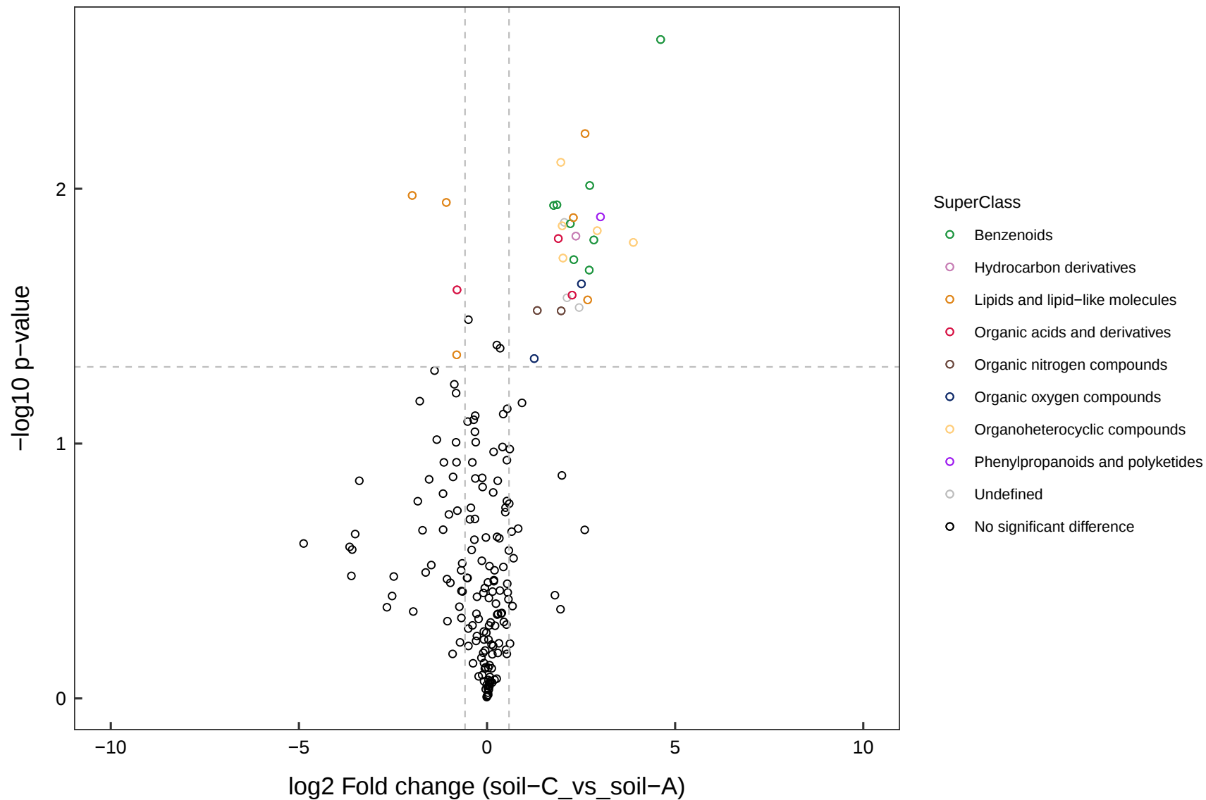
Volcano Plot
