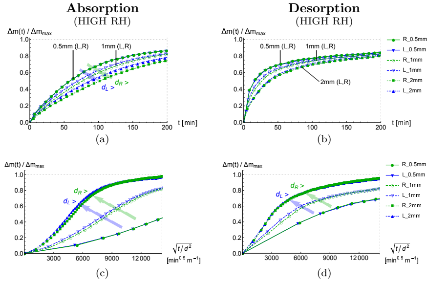
Fig. S3: Comparison of the sorption kinetics between samples with a different thickness in the longitudinal (blue) and radial (green) direction in the high range of RH. Absorption kinetics (80% → 90% RH) are shown left (a,c) and desorption kinetics (90% → 80% RH) right (b,d). Error bars were omitted for a better comparability and the interpolated lines are for illustration purposes only
