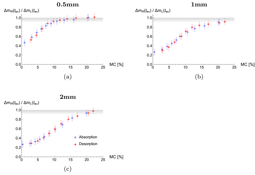
Fig. S4: Initial mass change ratio between radial and longitudinal samples during absorption (★) and desorption (◆) for a sample thickness of 0.5 mm (a), 1 mm (b), and 2 mm (c). Grey area indicates the range with a similar sorption kinetic between the radial and longitudinal samples
