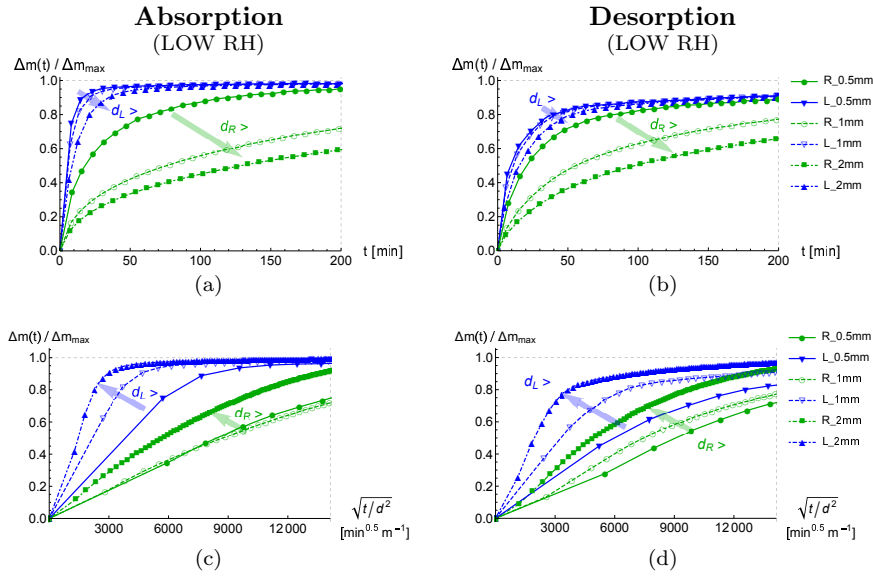
Fig. S2: Comparison of the sorption kinetics between samples with a different thickness in the longitudinal (blue) and radial (green) direction in the low range of RH. Absorption kinetics (0% → 10% RH) are shown left (a,c) and desorption kinetics (20% → 10% RH) right (b,d). Error bars were omitted for a better comparability and the interpolated lines are for illustration purposes only
