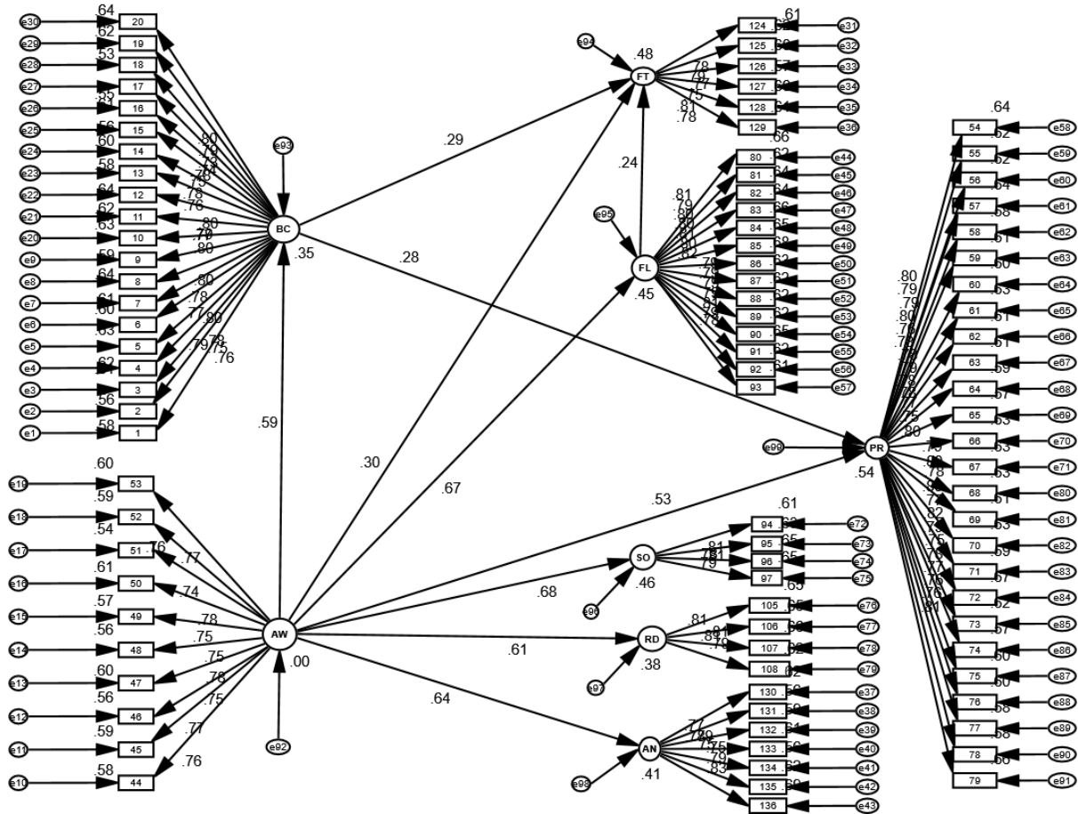
Figure 7. Final structural equation model with standardized factor loadings, standardized structural coefficients, and squared multiple correlations.
