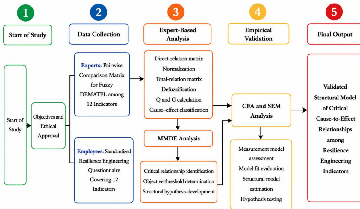
Figure 1. Overall analytical framework of the study, integrating expert-based fuzzy DEMATEL and MMDE analyses with employee-based CFA and SEM to identify and empirically validate critical relationships among resilience engineering indicators.
