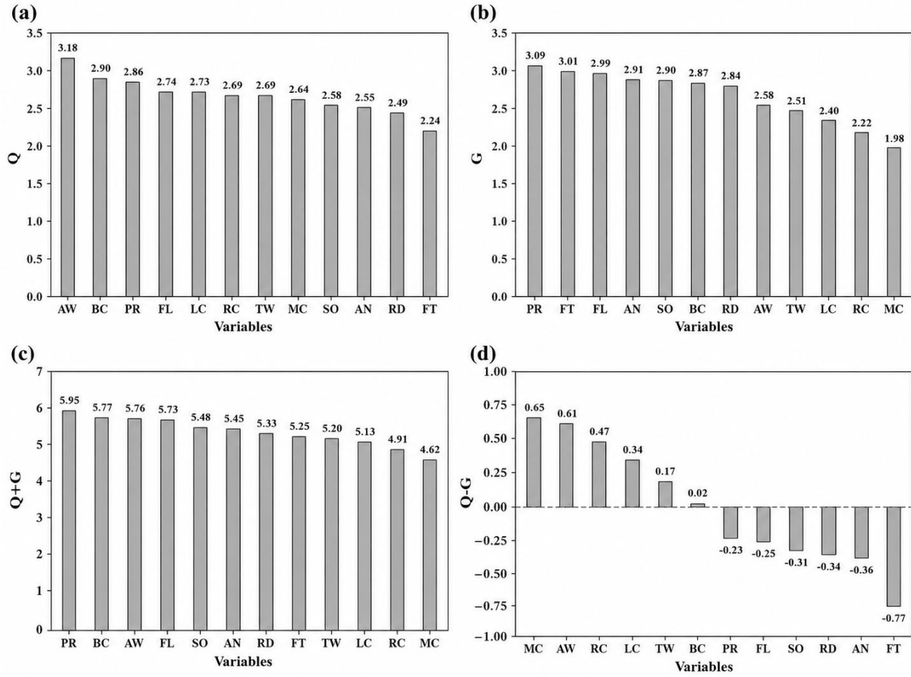
2 Figure 2. Results of the fuzzy DEMATEL analysis for the resilience engineering variables: (a) total 3 influence exerted ( Q_i ), (b) total influence received ( G_i ), (c) prominence ( Q_i + G_i ), and (d) relation ( Q_i 4 - G_i ). Positive values of Q_i - G_i indicate variables belonging to the cause group, whereas negative 5 values indicate variables belonging to the effect group.
