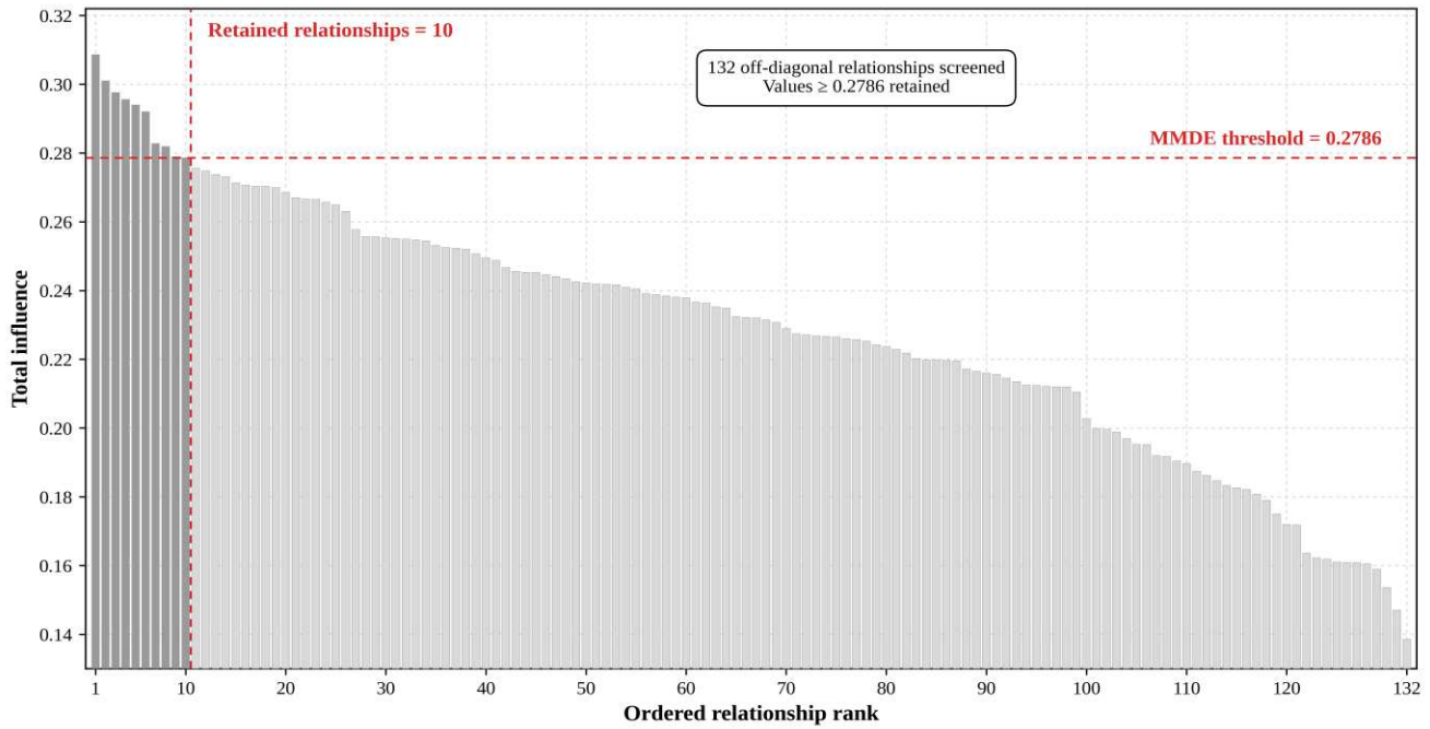
4 5 Figure 5. Ordered off-diagonal total-influence values and the MMDE threshold. The first 10 6 relationships met or exceeded the threshold of 0.2786, whereas the remaining 122 relationships were 7 excluded.
