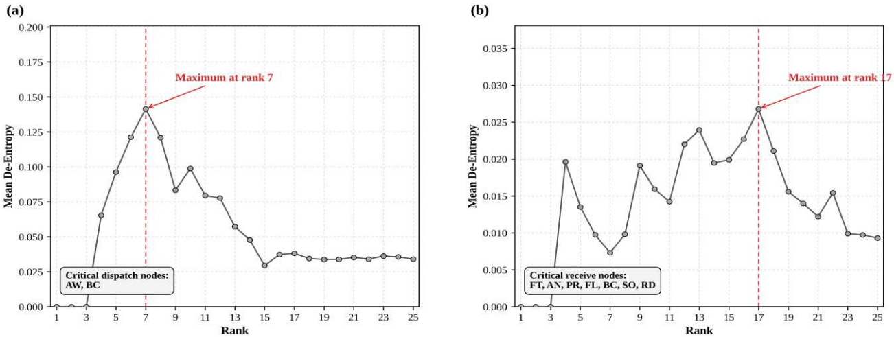
Figure 4. Mean de-entropy profiles used for MMDE relationship selection: (a) dispatch-node sequence and (b) receive-node sequence. The dashed red lines indicate the maximum mean de-entropy values at ranks 7 and 17, respectively.
