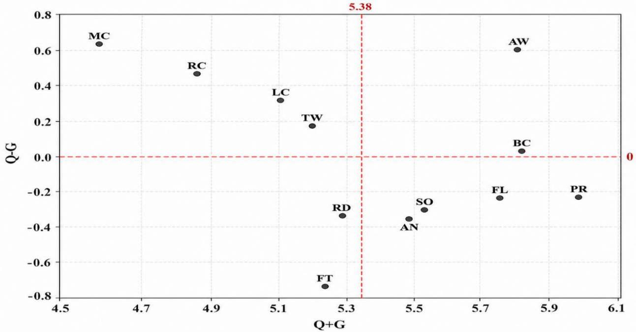
1 2 Figure 3. Cause–effect diagram of the resilience engineering variables based on fuzzy DEMATEL. The 3 horizontal axis denotes prominence ( Q_i + G_i ) and the vertical axis relation ( Q_i - G_i ); positive and 4 negative relation values identify cause and effect variables, respectively. The vertical dashed line 5 represents the mean prominence value of 5.381. 6 Table 6. DEMATEL influence indices and net-cause/net-effect classification of the resilience 7 engineering indicators
