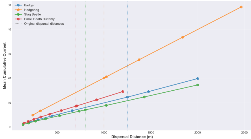
Sensitivity Analysis: All Species Comparison
