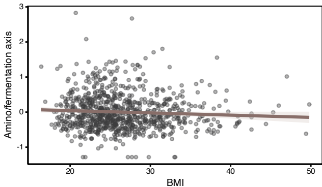
ZeeviD_2015: Amino/fermentation axis vs BMI
