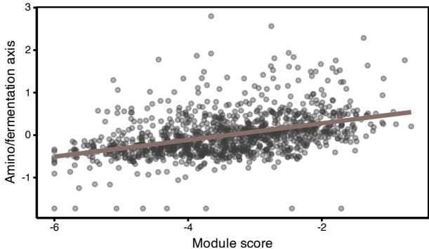
LifeLinesDeep_2016: Amino/fermentation axis vs module score
