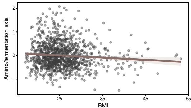
AsnicarF_2021: Amino/fermentation axis vs BMI
