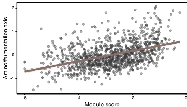
AsnicarF_2021: Amino/fermentation axis vs module score
