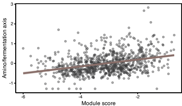
ZeeviD_2015: Amino/fermentation axis vs module score
