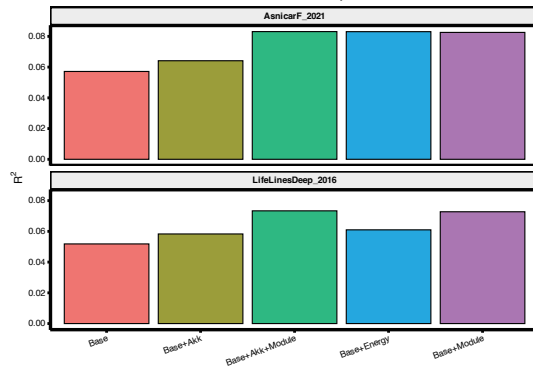
Incremental model comparison
