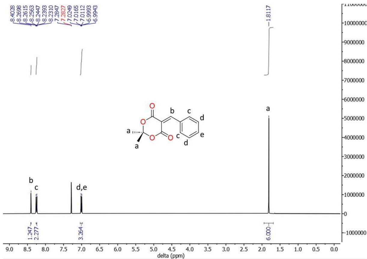
Figure S2: 1 H NMR spectra of 4 .
