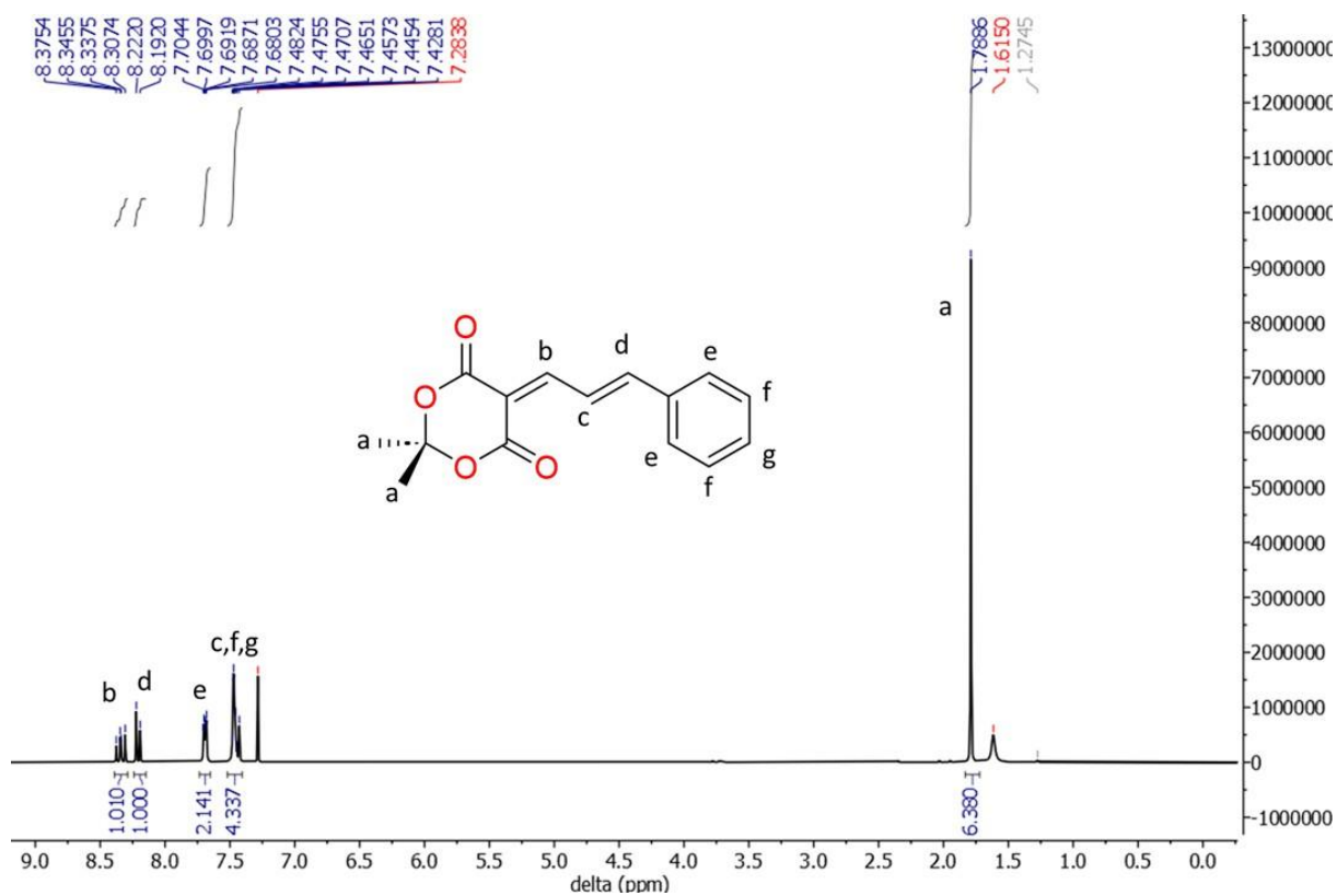
Figure S1: 1 H NMR spectra of 3 .
