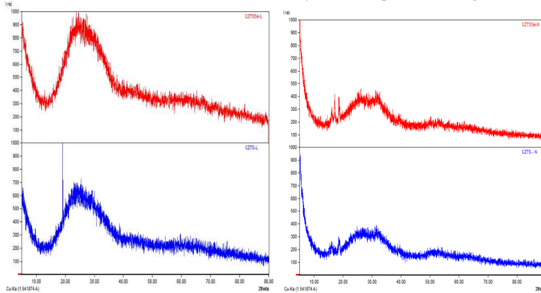
Figure 5. X-ray diffraction patterns of CZTS-L, CZTS-N, CZTSSe-L, and CZTSSe-N kesterite semiconductors
