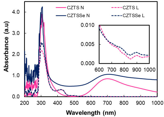
Figure 9. UV-Vis absorption spectrum of the synthesized kesterite solutions CZTS N, CZTS L, CZTSSe N, and CZTSSe L before calcination
