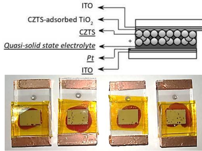
Figure 4. CZTS solar cell design (top) and TiO 2 /Cu 2 ZnSn(S,Se) 2 solar cell fabrication (bottom)
