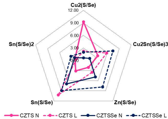
Figure 7. The net diagram of the secondary Phase of the kesterite semiconductor based on the analysis of the X-ray diffraction pattern of the semiconductor using the reference intensity ratio (RiR) method
