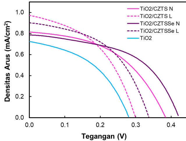
Figure 12. I-V characteristics of CZTS N, CZTS L, CZTSSe N, CZTSSe L, and \text{TiO}_2 solar cells
