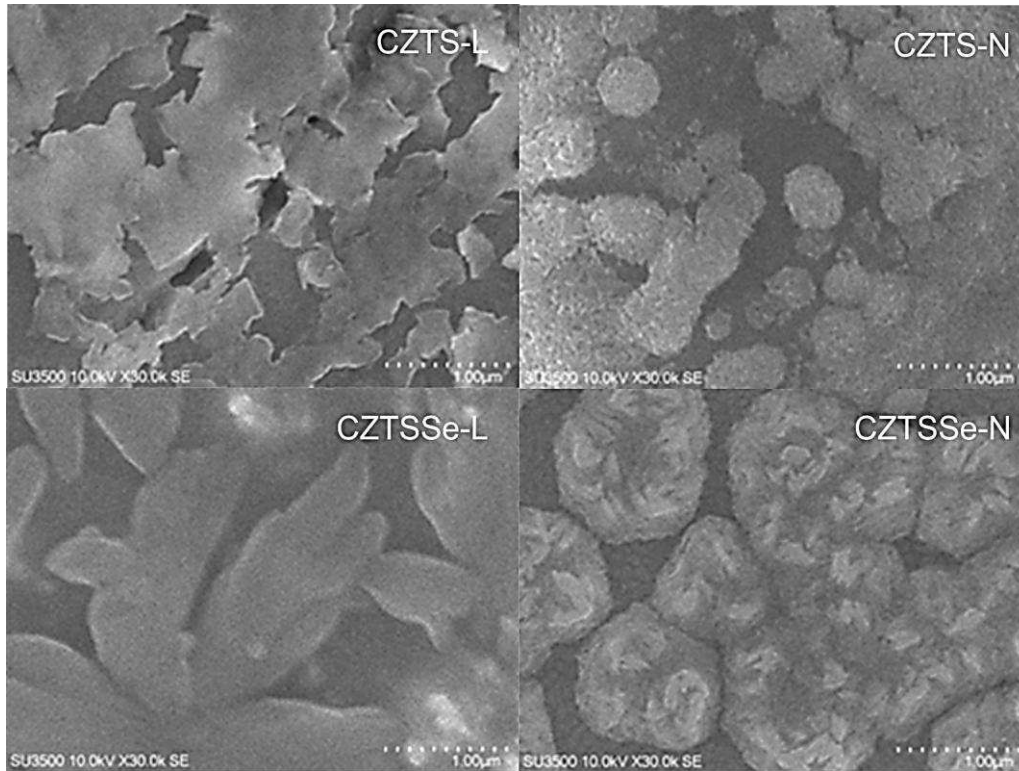
Figure 8. Scanning electron microscope (SEM) photo of the crystalline film surface (a) CZTS-L, (b) CZTS-N, (c) CZTSSe-L, (d) CZTSSe-N with 30,000 times magnification
