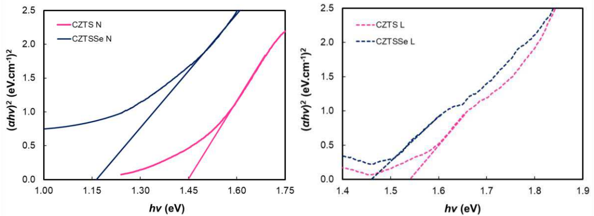
Figure 11. Graph of direct bandgap analysis of CZTS N, CZTS L, CZTSSe N, and CZTSSe L crystals based on Tauc's plot analysis
