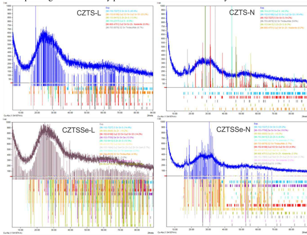
Figure 6. X-ray diffraction pattern analysis of CZTS-L, CZTS-N, CZTSSe-L, and CZTSSe-N semiconductors using the reference intensity ratio (RiR) method
