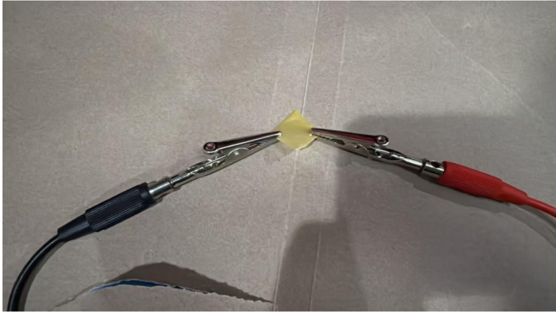
PEEK-3 Film Insulation Resistance Test
