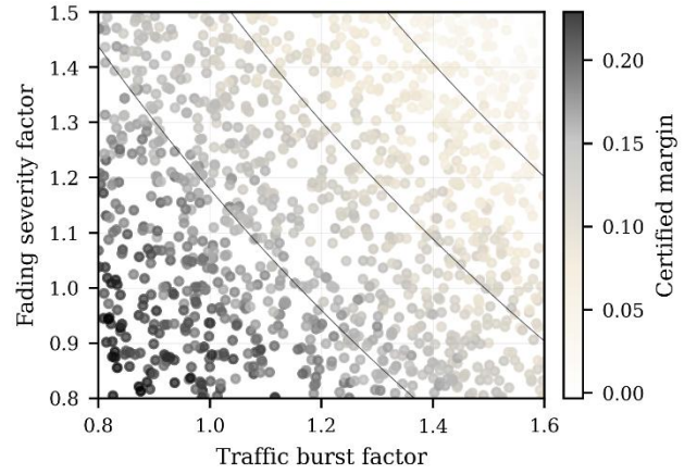
Fig. 12. Scenario-level certified margin under traffic-burst and fading-severity variations.
