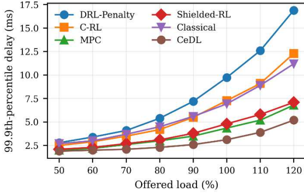
Fig. 4. URLLC tail-delay performance under increasing offered load.
