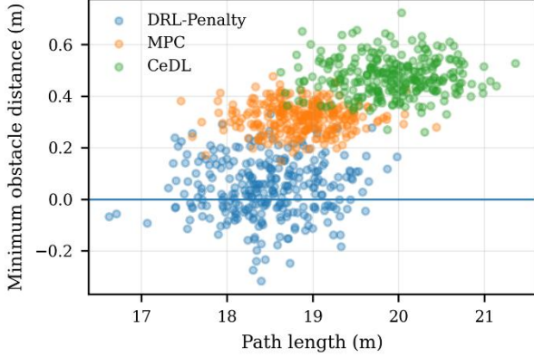
Fig. 9. Safety-efficiency tradeoff in robotic obstacle avoidance.
