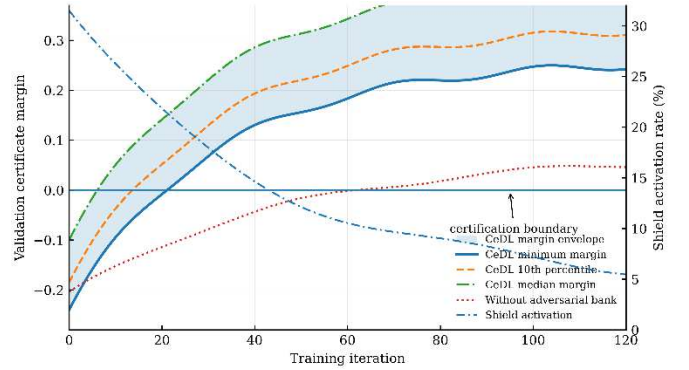
Fig. 2. Counterexample-guided improvement of certificate margins during training. The proposed CeDL procedure improves the minimum and lower-tail validation margins while reducing the need for runtime shield activation.
