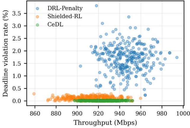
Fig. 10. Throughput-reliability tradeoff in URLLC resource allocation.
