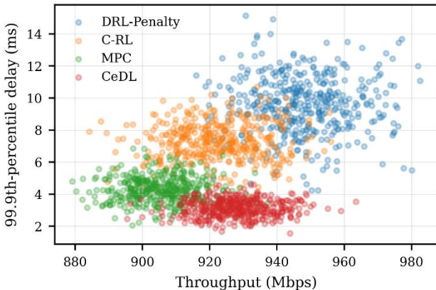
Fig. 11. Tail-delay and throughput tradeoff under URLLC operation.
