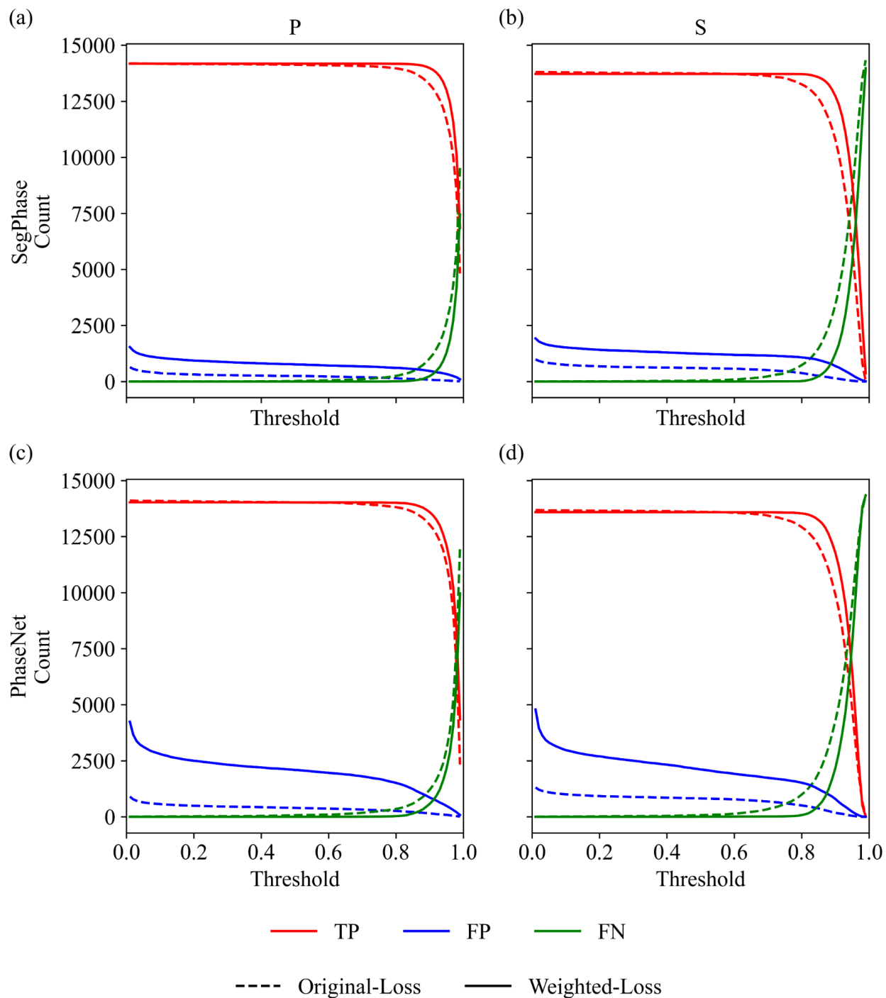
Figure 1. Threshold dependence of true-positive, false-positive, and false-negative counts. Threshold-dependent numbers of true positives (TP), false positives (FP), and false negatives (FN) for P- and S-wave picks. Panels (a) and (b) show the results for SegPhase P- and S-wave picks, respectively, and panels (c) and (d) depict the corresponding results for PhaseNet, respectively. Red, blue, and green curves indicate TP, FP, and FN counts, respectively. Solid and dashed lines indicate the weighted- and original-loss models, respectively.
