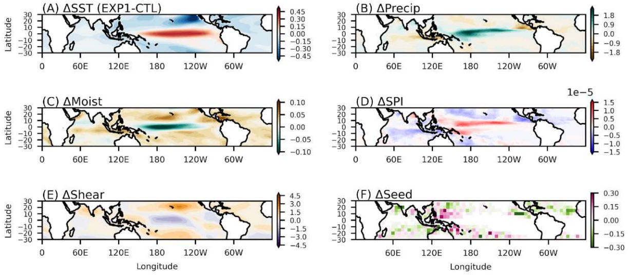
Figure 6. Difference in environmental conditions and seeds from CTL to EXP1. (A) Sea surface temperature, (B) precipitation, (C) saturation moisture deficit, (D) seed propensity index based on vorticity and precipitation, (E) vertical windshear, and (F) seed genesis density.
