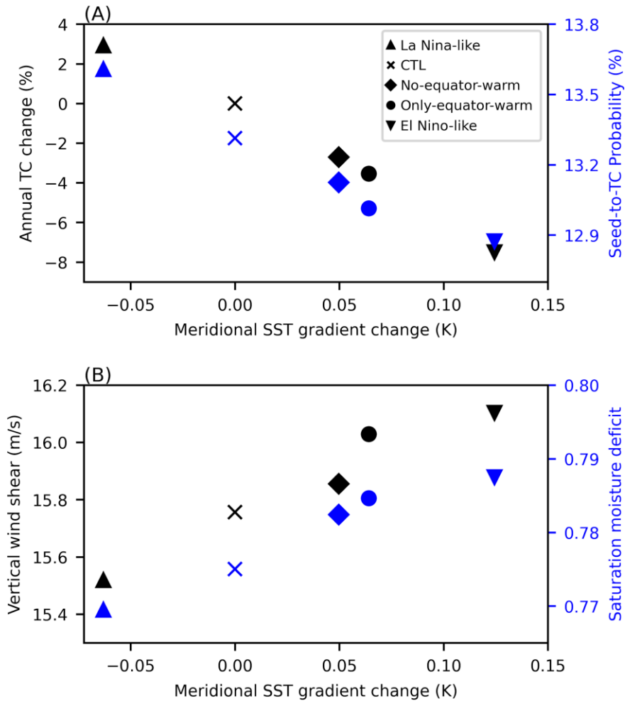
Figure 7. Summary of the global TC and environmental conditions from each SST experiment. The X-axis represents the meridional SST gradient change from the control run, calculated from the change in SST of the equatorial region (10°S-10°N) minus the change in SST in the off-equatorial region (10-30°N/S) compared to the control run. (A) The Y-axis on the left (black) represents the annual TC number change from the control simulation, and the Y-axis on the right (blue) represents the Seed-to-TC probability. (B) The Y-axis on the left (black) represents the vertical wind shear, and the Y-axis on the right (blue) represents the saturation moisture deficit. The global mean of each quantity on the Y-axis excludes 5°S-5°N and the Southeastern Pacific and South Atlantic regions, where TC activity is rare.
