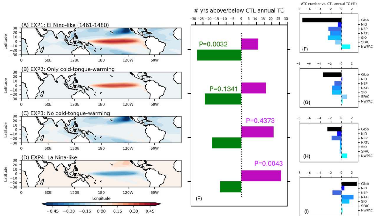
Figure 3. Idealized sea surface temperature (SST) experiments and tropical cyclone response. (A-D) The mean SST difference compared to the control simulation (CTL) (1401-1420): (A) Experiment 1: averaged SST between 1461-1480 (El Niño-like), (B) Experiment 2: only cold-tongue-warming, (C) Experiment 3: no cold-tongue-warming, and (D) Experiment 4: La Niña-like. (E) The number of years that the tropical cyclone (TC) counts in each experiment are above (magenta bar) or below (green bar) the mean value of the TC counts in CTL. P-value for the binomial test is displayed. (F-I) The percentage change in the mean of TC number from CTL to each experiment globally (black bar) and in each basin (different blue bars). The percentage change in each basin is relative to the mean global TC number in CTL.
