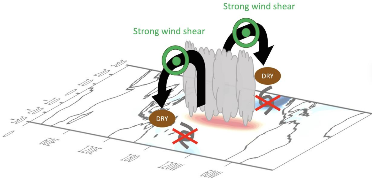
Figure 8. Schematic of the decrease in global TC frequency under an El Niño-like SST trend. Equatorial warming induces stronger meridional circulation, stronger wind shear, and a drier midtroposphere, which are detrimental to TC genesis
