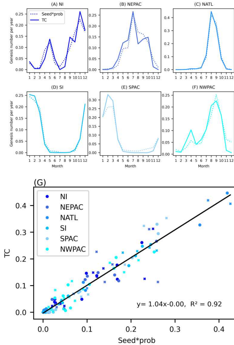
Figure 4. Annual cycle of actual TC number and estimated TC number (i.e., seed multiplied by transition probability) after normalization. (A-F) Annual cycle of actual TC number (solid line) and estimated TC number (dotted line) in the control run in each basin: (A) North Indian Ocean (NI), (B) North Eastern Pacific (NEPAC), (C) North Atlantic (NATL), (D) Southern Indian Ocean (SIO), (E) Southern Pacific Ocean (SPAC), and (F) North Western Pacific (NWPAC). (G) Scatter plot between the annual cycle of the actual (y-axis) and estimated (x-axis) TC number for each basin. Dots represent the control run, while crosses represent Experiment 1. The linear regression line is displayed.
