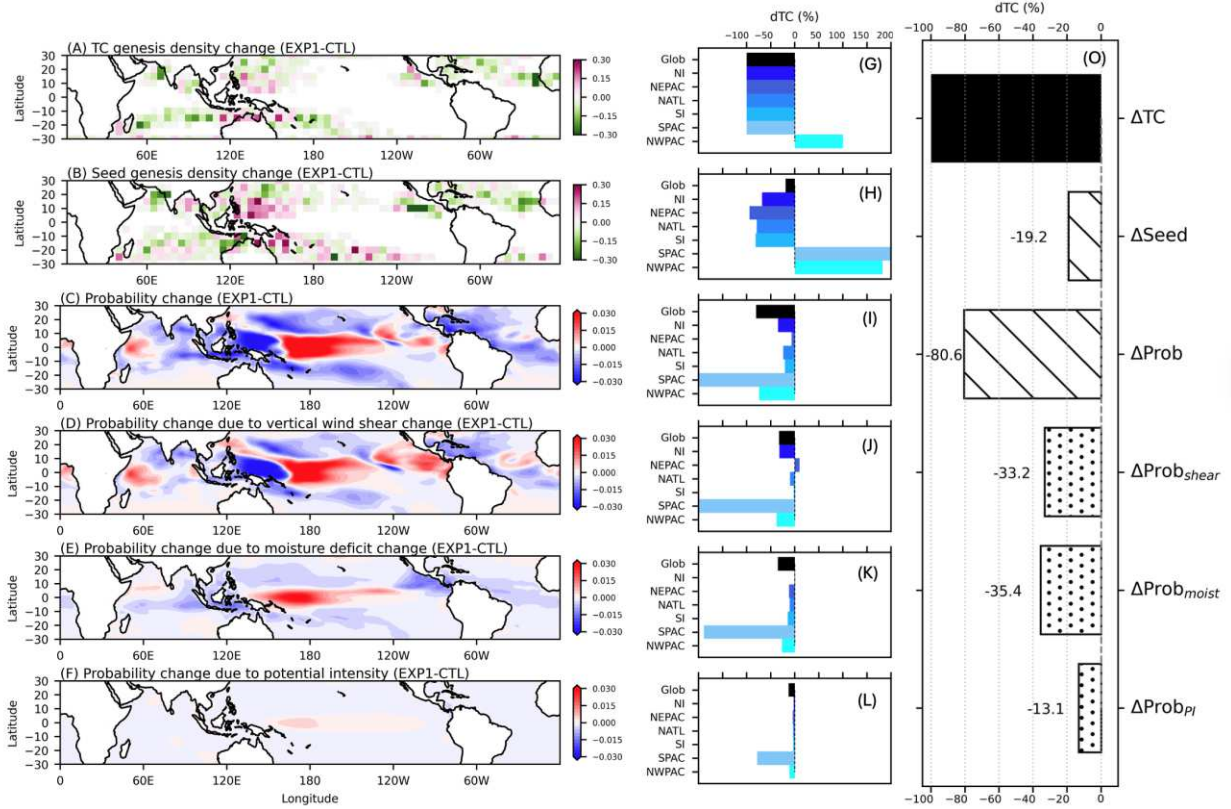
Figure 5. Difference in seed and probability from CTL to EXP1. (A) The genesis density of tropical cyclones, (B) the genesis density of seeds, (C) the calculated transition probability from seed to tropical cyclones based on potential intensity, saturation moisture deficit, and vertical wind shear, (D-F) the calculated transition probability with a single variable in Experiment 1, while the other environmental factors are kept the same as in CTL. The single varying factor is: (D) potential intensity, (E) saturation moisture deficit, (F) vertical wind shear. (G-L) The percentage change of TC genesis number from CTL to Experiment 1 in each basin due to each factor: (G) actual TC number change, (H) seed density change, (I) probability change, (J) potential intensity change that changes probability, (K) saturation moisture deficit change that changes probability, (L) vertical wind shear change that changes probability. (O) The percentage change of the global TC number (solid bar) due to changes in seeds and probability (slanted hatch). The change in probability can be separated by changes in shear, moisture, and potential intensity (dotted hatch).
