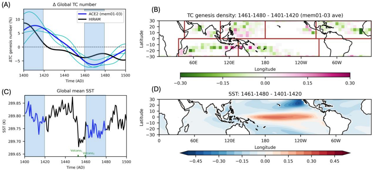
Figure 1. Changes in global TCs and SSTs in the 15 th century. (A) Time series of the percentage change of global tropical cyclone numbers from 1401 to 1500. The light blue lines represent each ACE2-ERA5 ensemble member, with the dark blue line representing the ensemble mean. The black line represents the hurricane-level tropical cyclones in HiRAM. (B) The change in genesis density of tropical cyclones from 1401-1420 to 1461-1480 averaged across three ensemble members. The red box marks each basin. The top row from left to right represents the North Indian Ocean (NIO), the North Western Pacific (NWPAC), the North Eastern Pacific (NEPAC), and the North Atlantic (NATL), while the bottom row represents the South Indian Ocean (SIO) and the South Pacific (SPAC). (C) The global mean sea surface temperature time series from 1401 to 1500. The green horizontal lines at the bottom indicate the two volcanic eruptions in 1452-1453 and 1459-1460. (D) The change in mean sea surface temperature from 1401-1420 to 1461-1480. The light blue shadings in (A) and (C) represent the High and Low periods we focus on in this study, depicting higher and lower TC numbers in the 15 th century.
