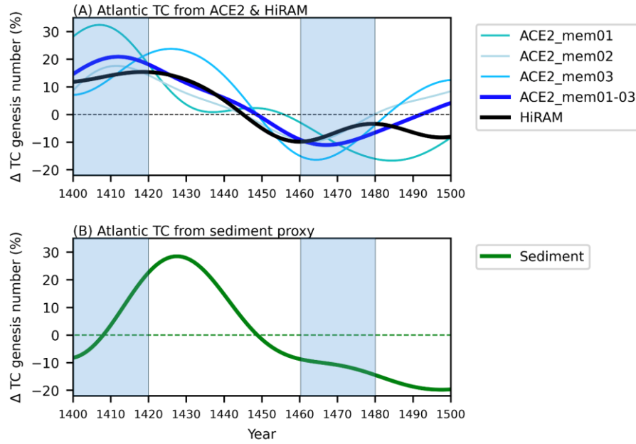
Figure 2. Time series of Atlantic tropical cyclone (TC) number change in the 15th century. (A) The light blue lines represent each ACE2-ERA5 ensemble member, with the dark blue line representing the ensemble mean. The black line represents the hurricane-level tropical cyclones in HiRAM. The light-blue shading represents the High and Low periods. (B) The green line represents the sediment proxy TC anomalies. TC anomalies from each data are applied with a 40-year low-pass filter.
