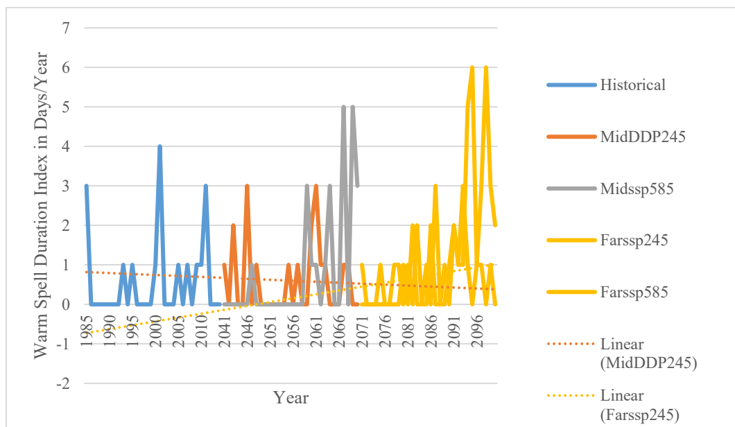
Figure 9 Trend of WSDI in Chewbet station from Historical to Projection periods Using CNRM Model
