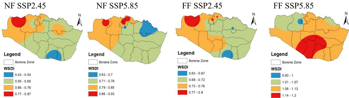
Figure 8 Spatial Variation of WSDI in Near Future and Far Future over the Study Area
