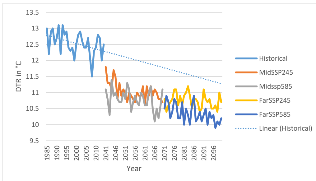
Figure 6 Trend of Diurnal Temperature Range at Chewbet Station Historical and Future CNRM Data
