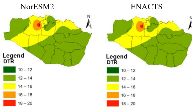
Figure 4 Spatial characteristics of Historical Diurnal Temperature Range (DTR) over Borana Zone
