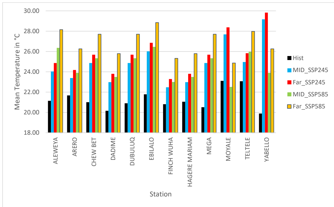
Figure 3 Mean Temperature Climatology from Historical, Near Future NF (MID) and Far Future (FF) Over Borana Zone
