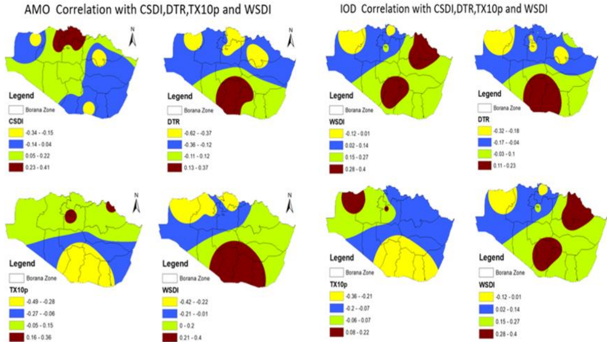
Figure 10 Spatial correlation coefficients of AMO (Left) and IOD (Right) with Temperature Extremes
