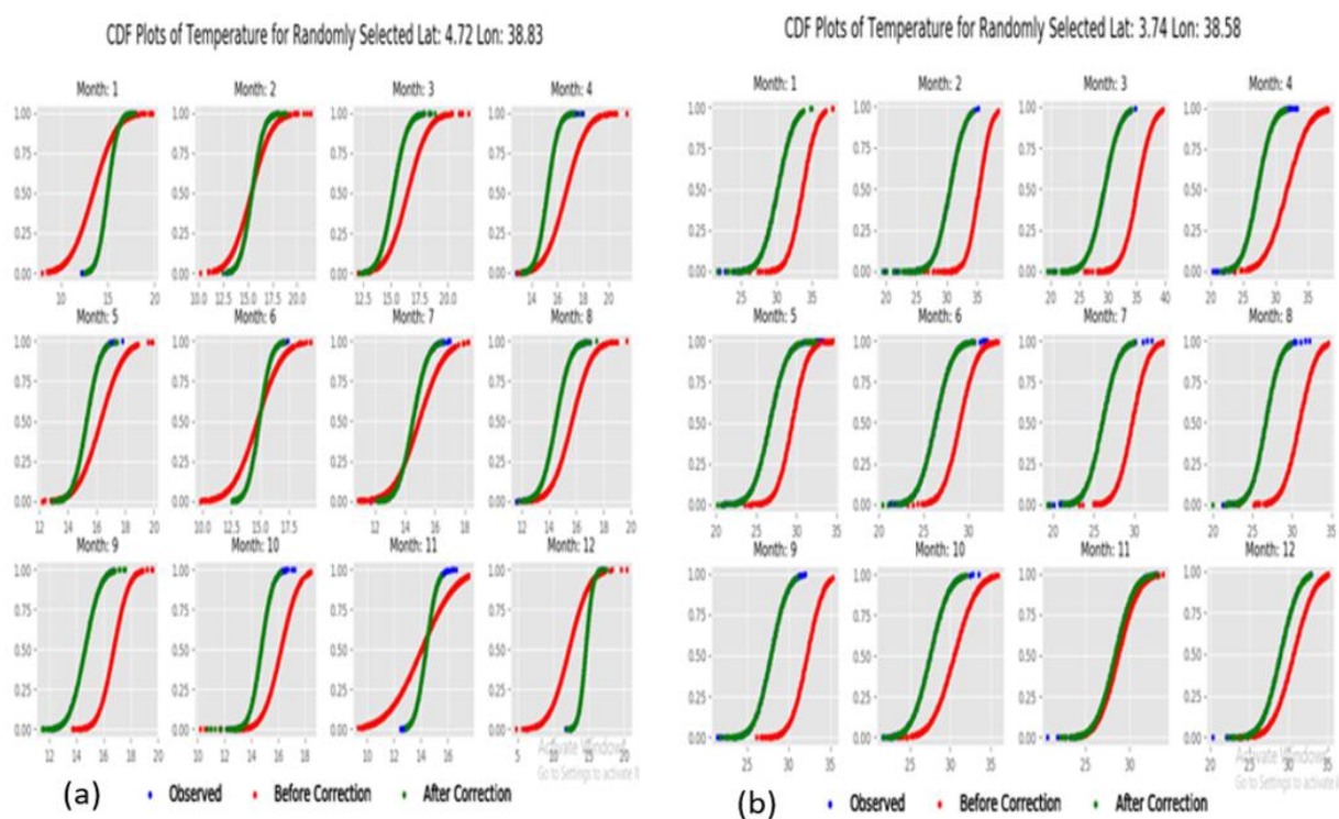
Figure 2 Cumulative distribution function (CDF) of the minimum (a) at Arero and maximum (b) temperatures and Ebilalo stations, respectively
