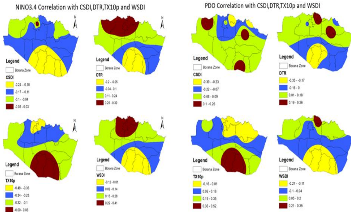
Figure 11 Spatial correlation coefficients of NINO3.4 (Left) and PDO (Right) with Temperature Extremes
