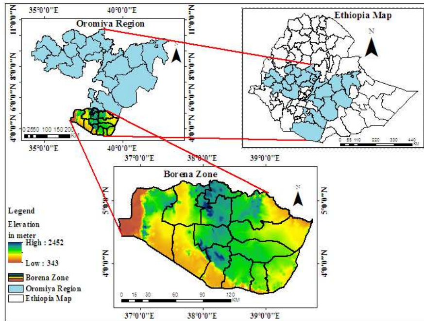
Figure 1 Map of the Study area with elevation
