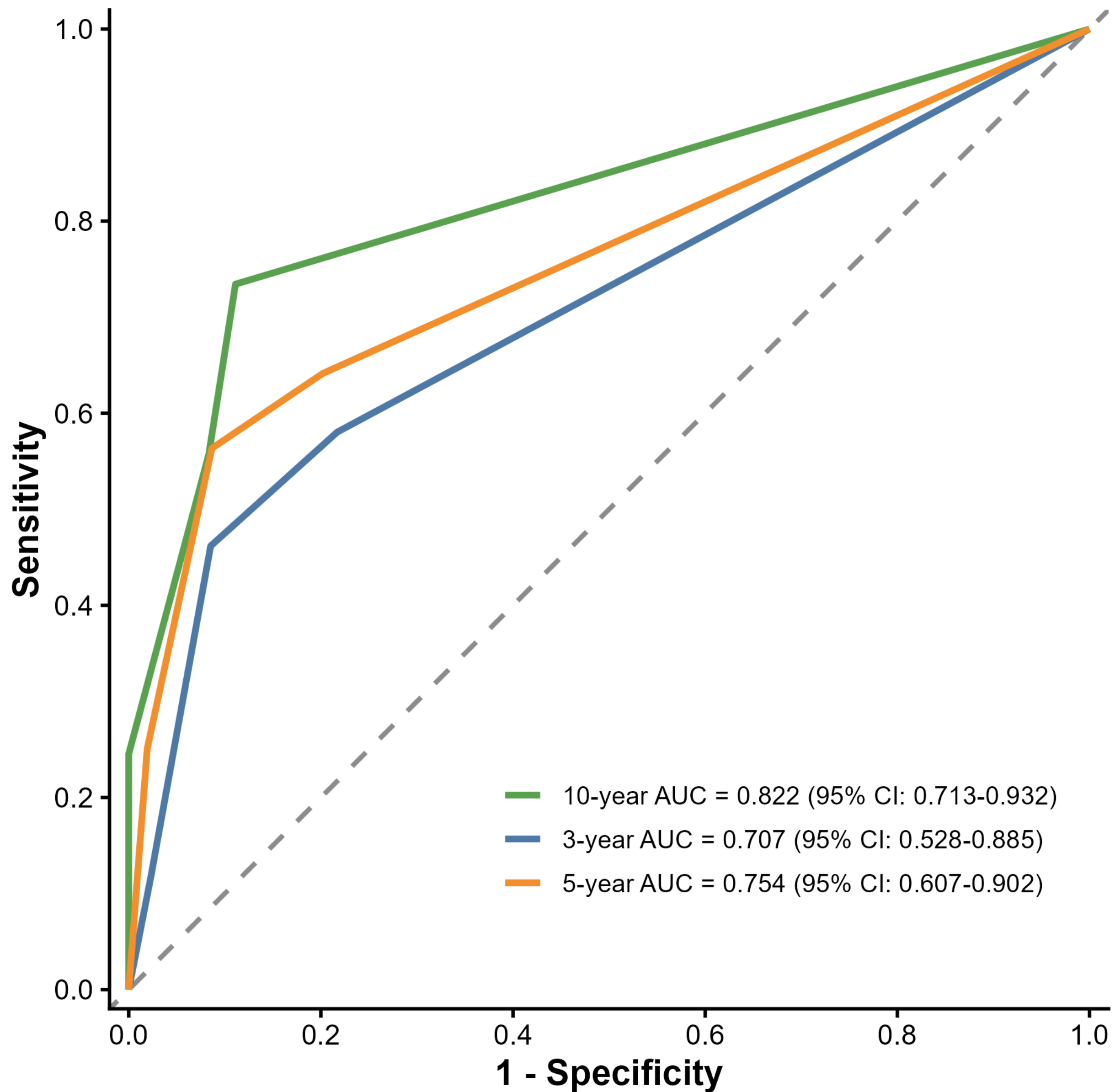
Training cohort: 3-/5-/10-year time-dependent ROC
