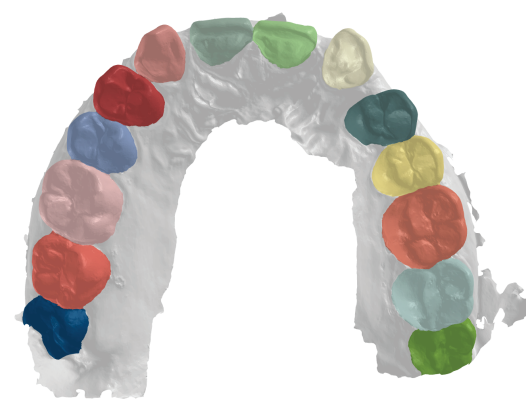
Case 9. DC-Net
