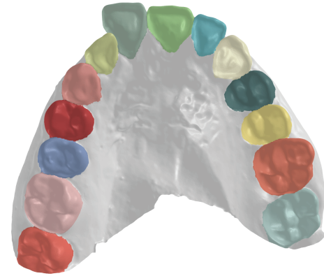
Case 7. DC-Net
