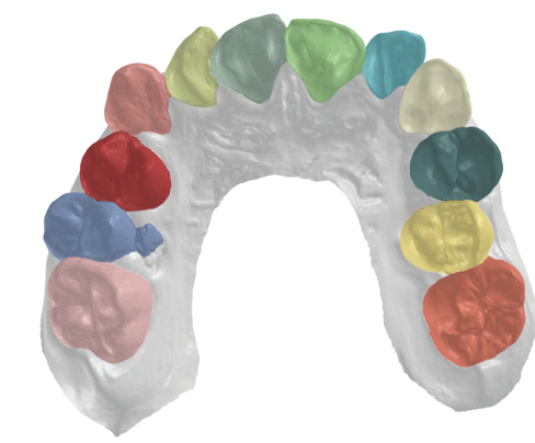
Case 8. DC-Net
