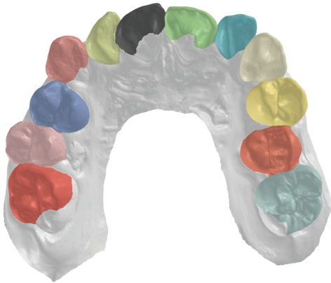
Case 8. Baseline
