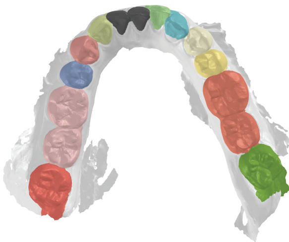
Case 10. Baseline
