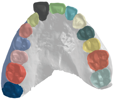
Case 7. Baseline
