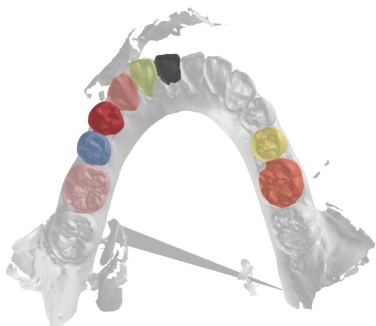
Case 5. Baseline
