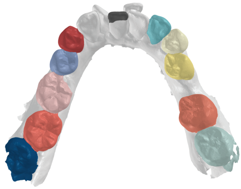
Case 2. Baseline
