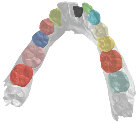
Case 3. Baseline
