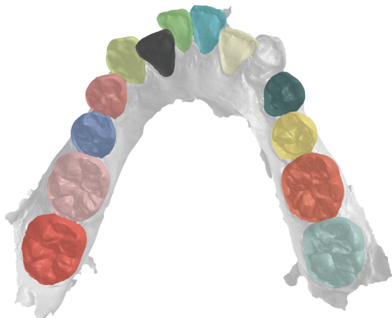
Case 4. Baseline
