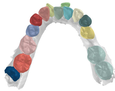
Case 2. DC-Net
