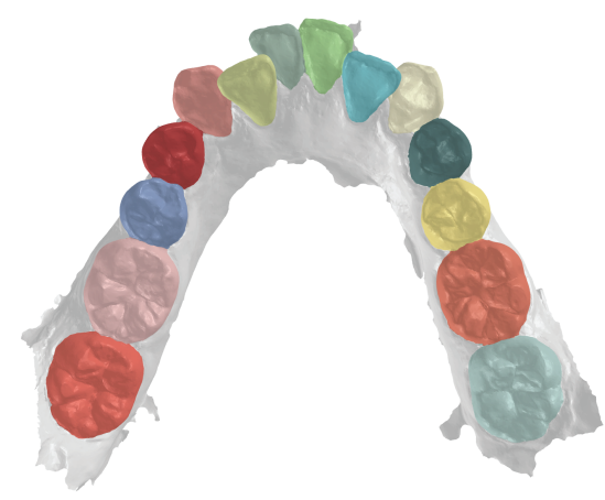
Case 4. DC-Net
