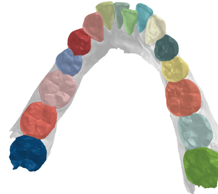
Case 3. DC-Net
