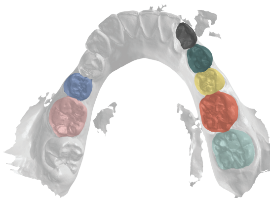
Case 4. Baseline
