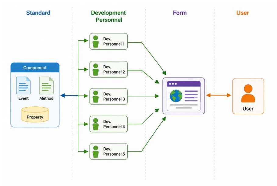
Figure 8 Attainment of user-interface consistency
