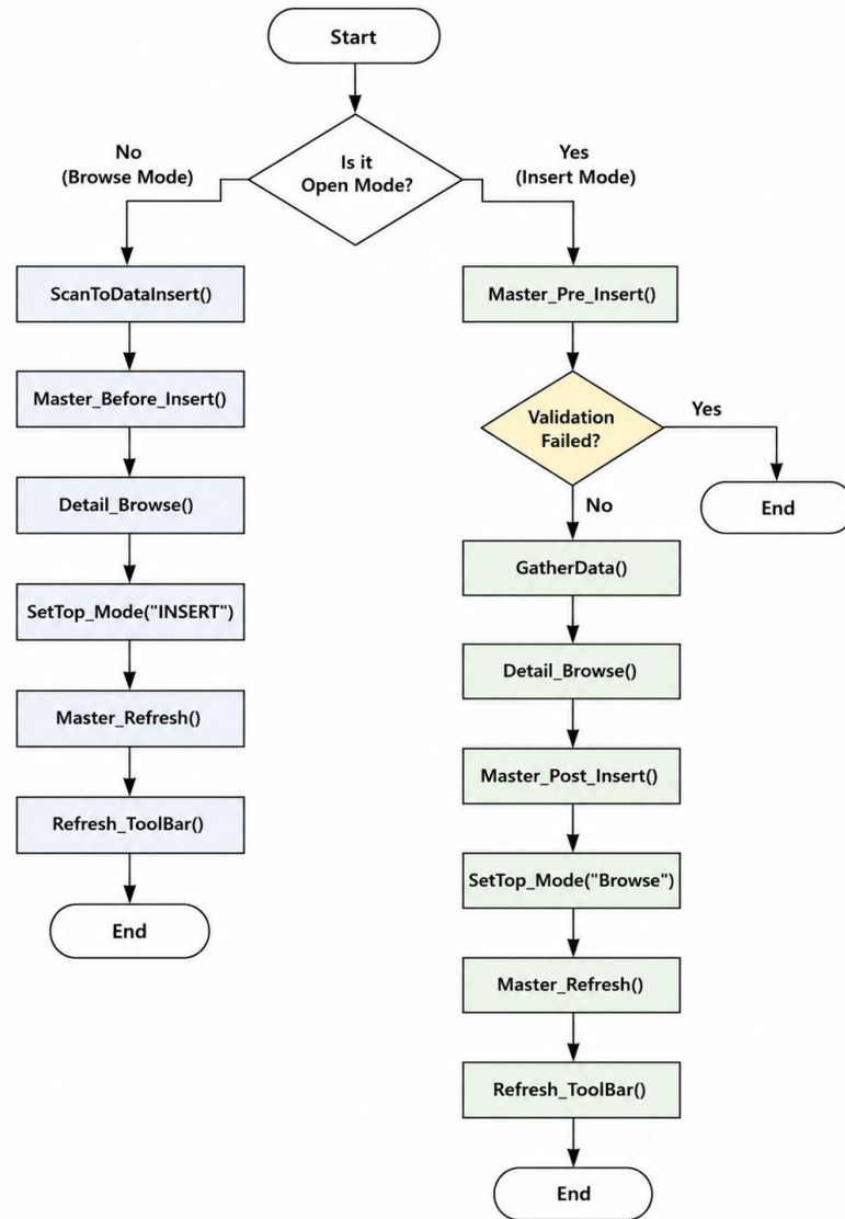
Figure 3 Button [Insert] event-driven flow chart
