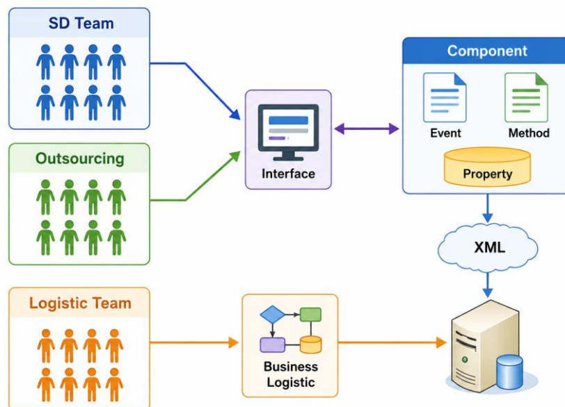
Figure 7 Attainment of collaborative development and security control
