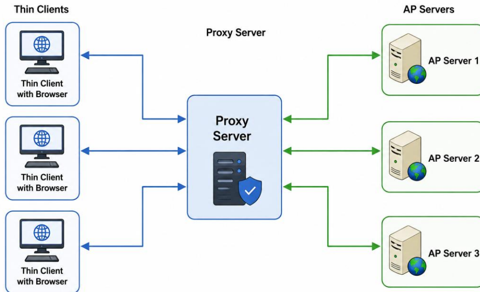
Figure 4 Solution to programming deployment and conflict
