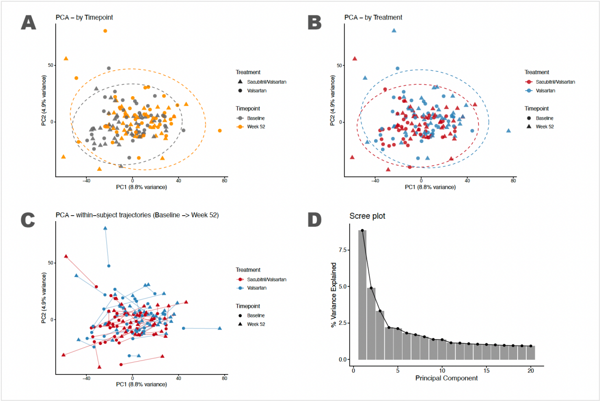
Extended Data Fig. 1: Principal component analysis (PCA) of full expression matrix.
