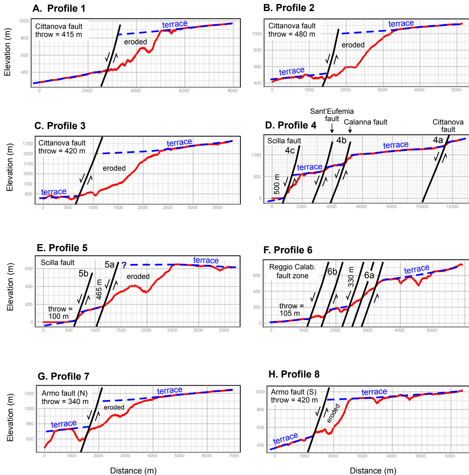
Supplementary Figure 5. Fault-throw profiles for major active normal faults in the study area. Red lines are topography; blue dashed lines are variably incised marine terraces. Profile locations are shown in Fig. 4. Calculated fault-throw rates vary from 0.8 to 4.2 mm yr -1 (see Table 1).
