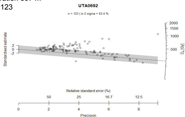
Supplementary Figure 1. Radial plots (left) and KDE plots (right) for 3 of the 6 samples with resolved luminescence ages. KDE is kernel density estimate. Dashed line in the radial plots is the D_e value from the minimum dose model, shaded gray area is \pm 2\sigma error.
