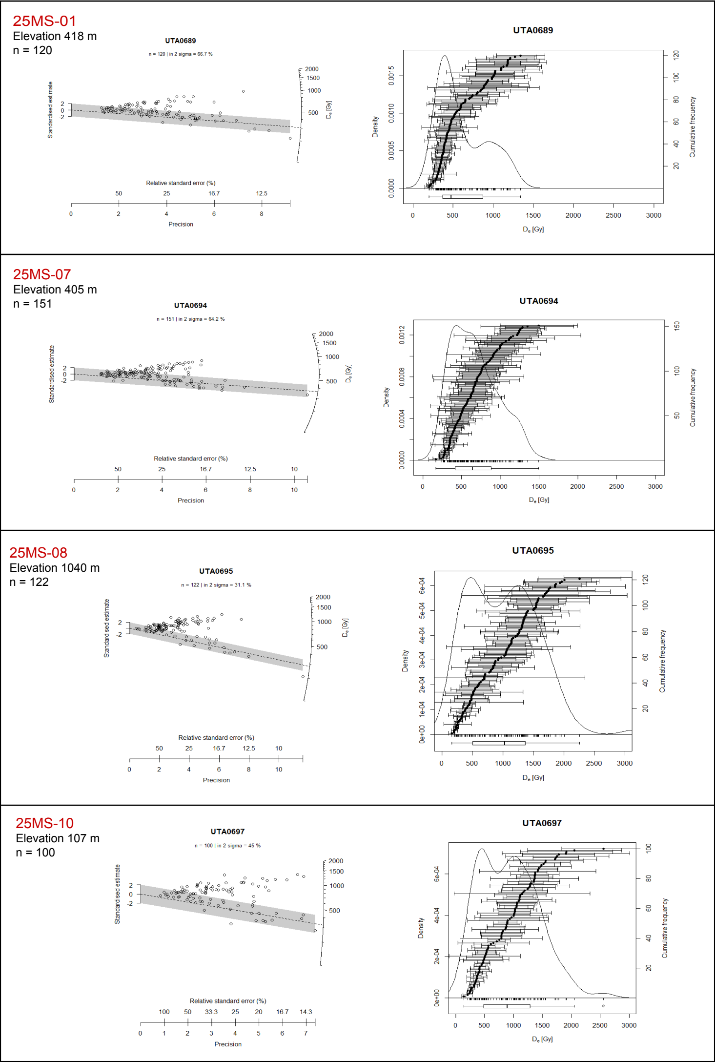
Supplementary Figure 3. Radial plots (left) and KDE plots (right) for the 4 samples with saturated (unresolved) luminescence ages. KDE is kernal density estimate. Dashed line in the radial plots is the De value from the minimum dose model, shaded gray area is \pm 2\sigma error.
