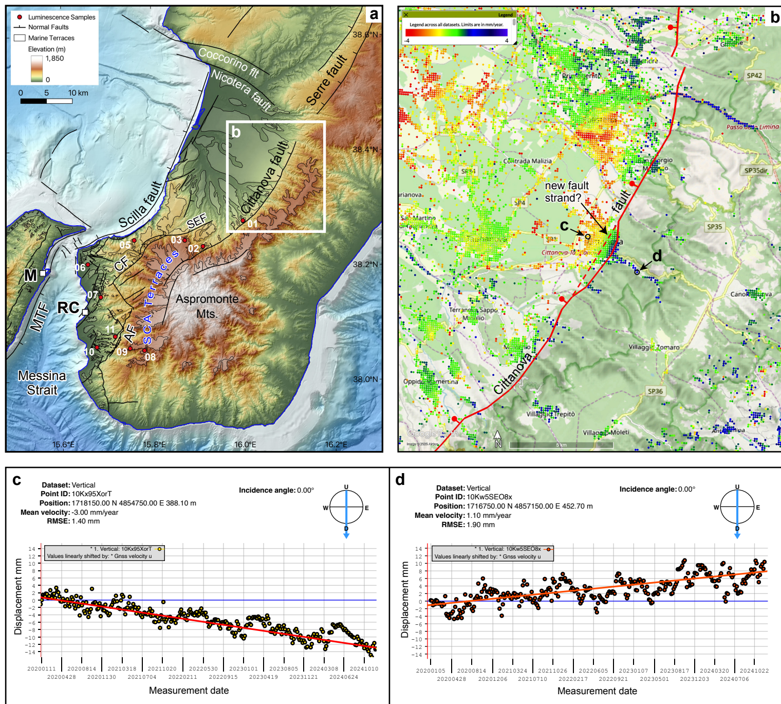
Supplementary Figure 6. Ground deformation in the vicinity of the Cittanova fault from the EGMS database (European Ground Motion Service: https://egms.land.copernicus.eu/ ). (a) Map modified from Fig. 1 showing location of map in b. (b) Map of the central to northern Cittanova fault showing the spatial pattern of vertical deformation derived from Sentinel-1 satellite data using the InSAR method. The data show a systematic change in vertical rate over a distance of ~1.5-2.5 km across the fault in several locations where data exist. Point locations for time series in c and d are shown. (c) Time series of vertical change for a representative point in the hanging wall of the Cittanova fault, mean velocity is -3.0 mm/yr. (d) Time series of vertical change for a representative point in the footwall of the Cittanova fault, mean velocity is +1.1 mm/yr. The difference in vertical rate between hanging wall and footwall locations over a period of 4 years is roughly 3.0–4.5 mm/yr, similar to the long-term post-120 ka fault-throw rate calculated for this fault (Table 1; Extended Data Fig. 5). The InSAR data also reveal unexplained variations that likely are related to complex interactions between short- and long-term deformation, changes in groundwater, surface mass movements, and human influence (e.g., ref 39). Similar variations in vertical motions along the Armo fault suggest a need for future work on this problem.
