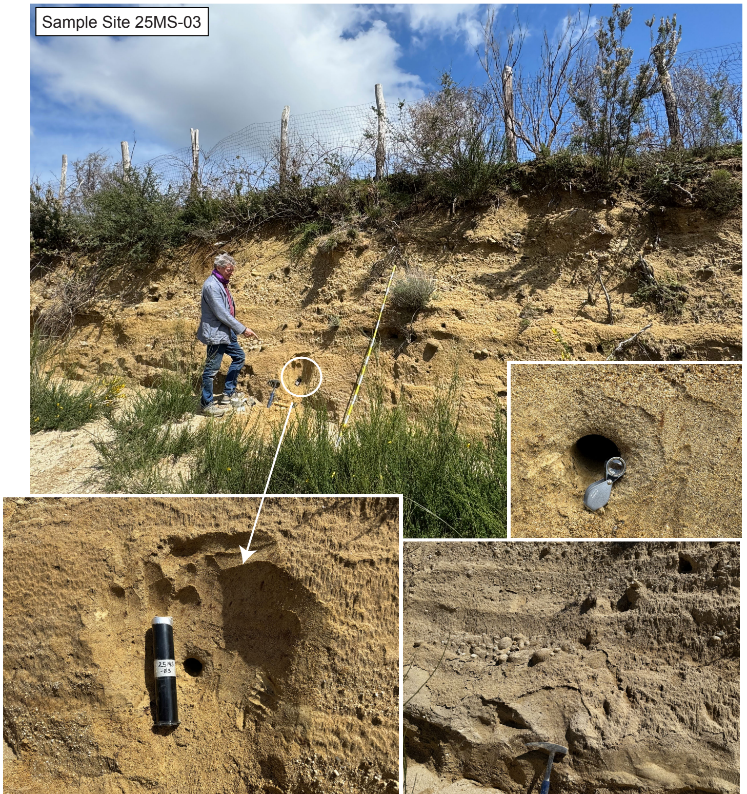
Supplementary Figure 8. Sample 25MS-03. lat 38.245610° / lon 15.871404°. Elevation 886 m. Overburden 2.5 m. Beach Sands unit of Jacques et al. (2001), ~2 km SE of Sant'Eufemia d'Aspromonte. Well sorted, very weakly cemented fine-grained massive sand interbedded with lenticular cross-stratified sands, very coarse granular sands, and small channels filled with well rounded pebble- to cobble-size granitic clasts (same as underlying basement rock near this location). Sample site is 2.5 m below vegetated terrace surface.
