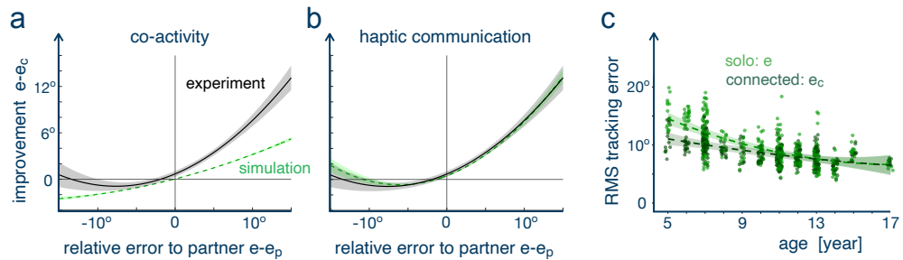
Fig. 3 Simulation of joint tracking in children. Experimental (black) and simulation (green) improvement with co-activity using only the mechanical connection (a) and with haptic communication (b). The central lines indicate the mean, and the shaded region the 95% confidence interval of the linear mixed effect model that best fits the data. c) Similar to the experimental results, simulated haptic communication yields tracking error that decrease with age and are further reduced when partners are connected.
