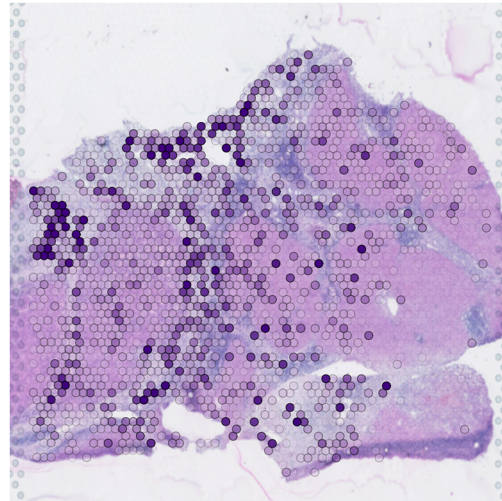
ECM-integrin context
