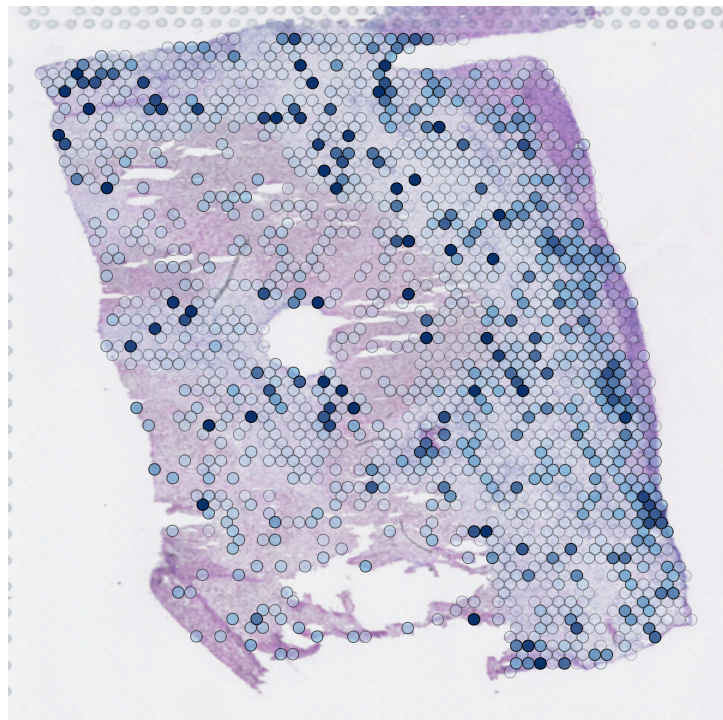
CD74/CXCR4
