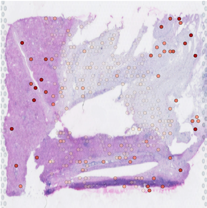
CD74/CXCR4
