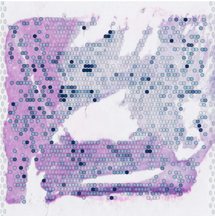
CD74/CXCR4
