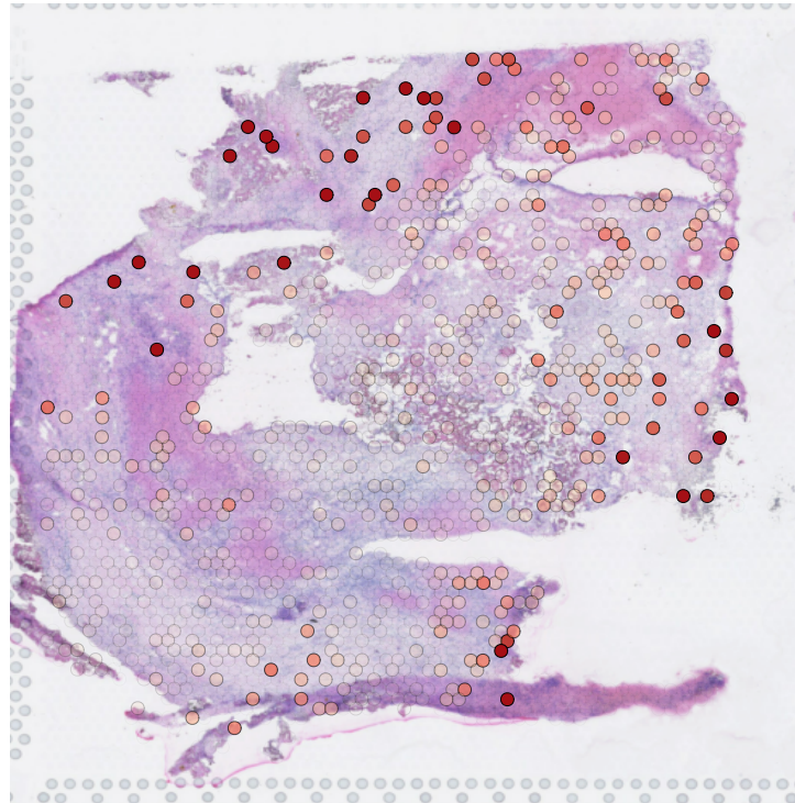
CD74/CXCR4
