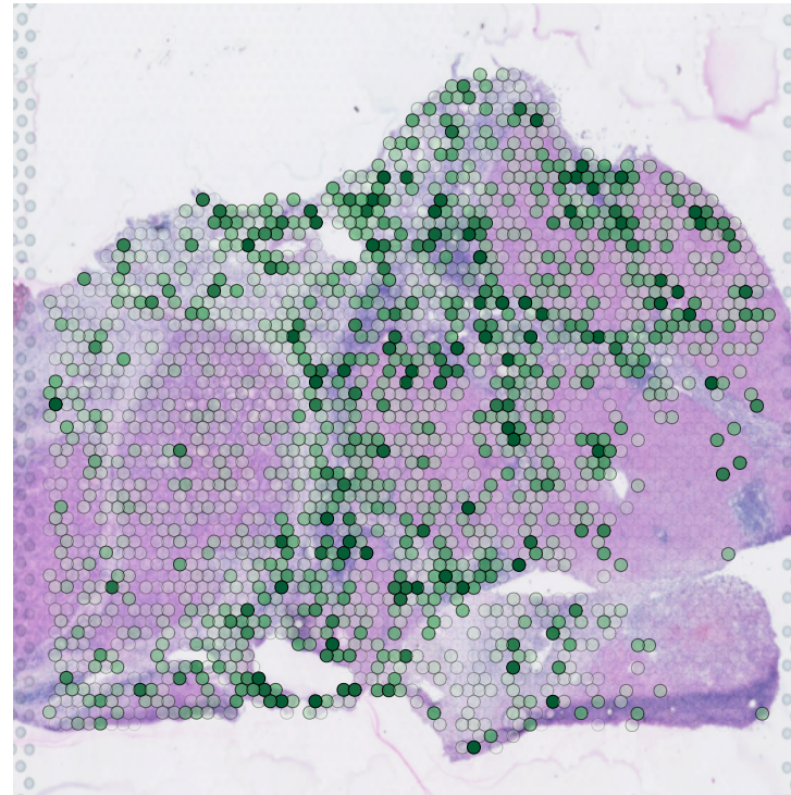
ECM-integrin context
