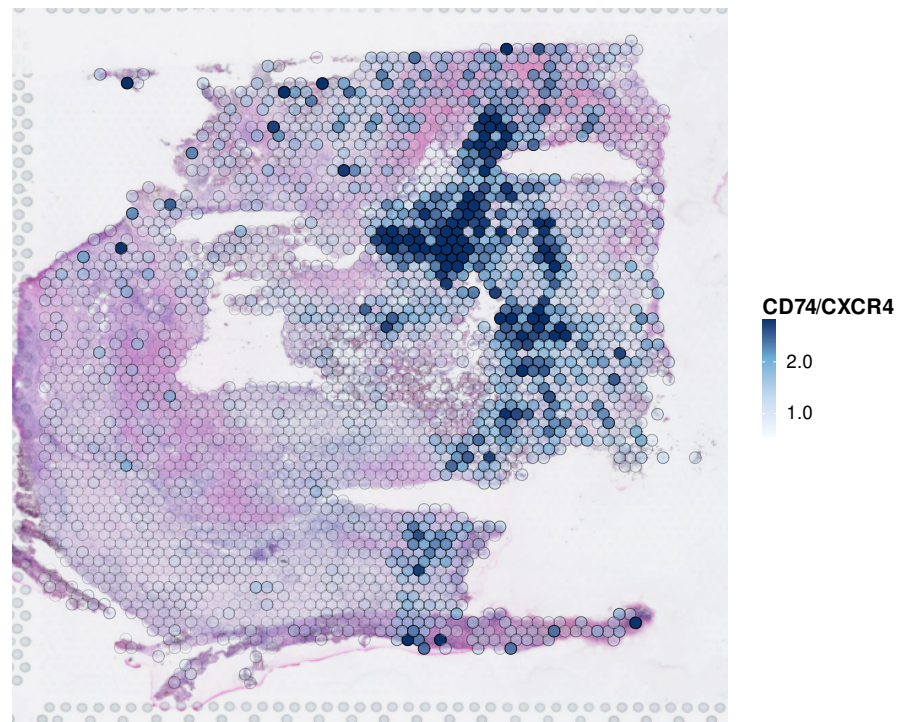
CD74/CXCR4
