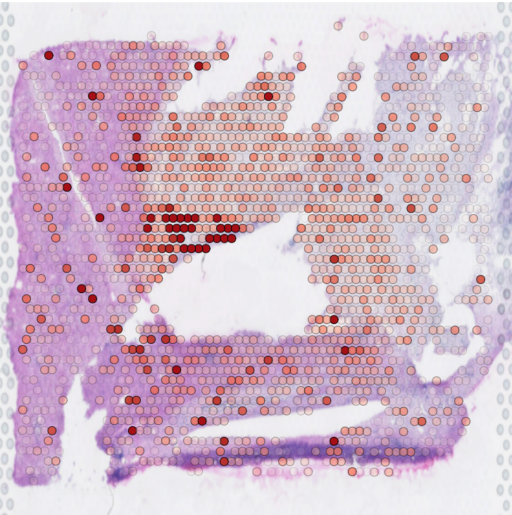
C3-like score
