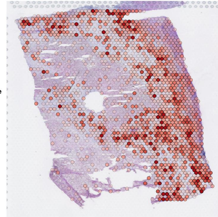
C3-like score
