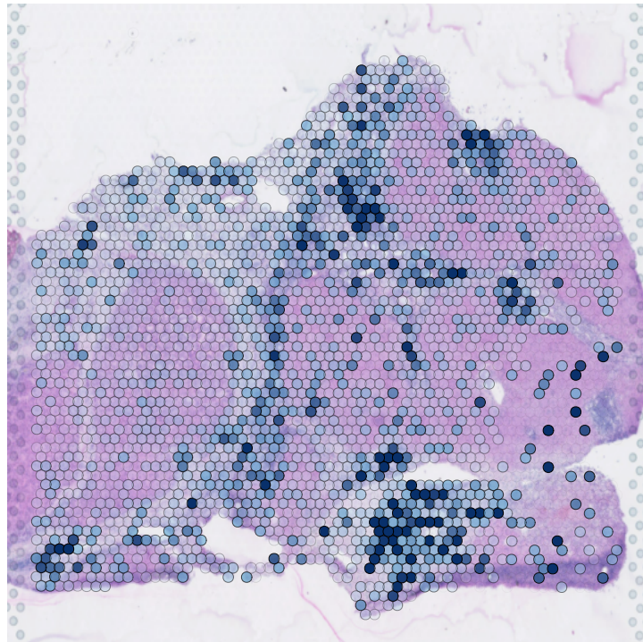
CD74/CXCR4
