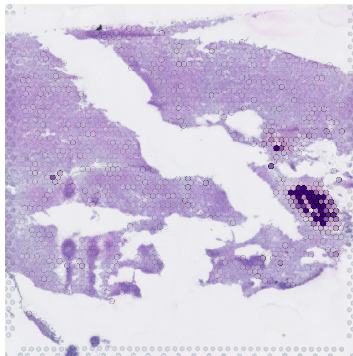
ECM-integrin context
