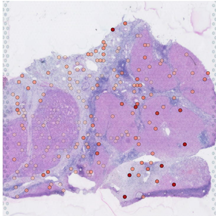
CD74/CXCR4
