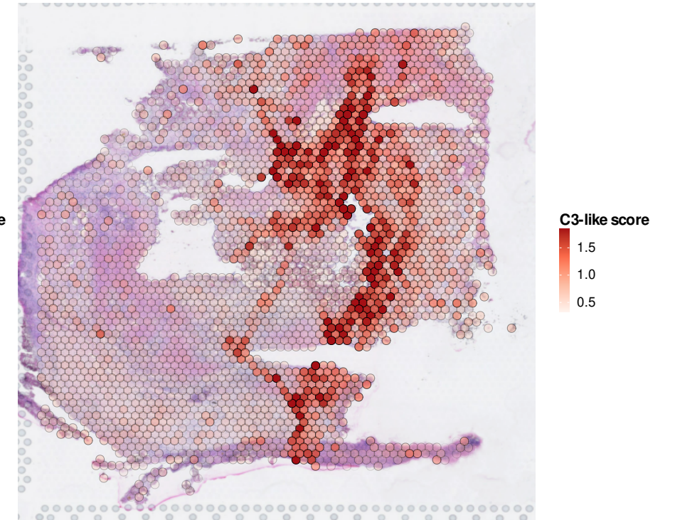
C3-like score
