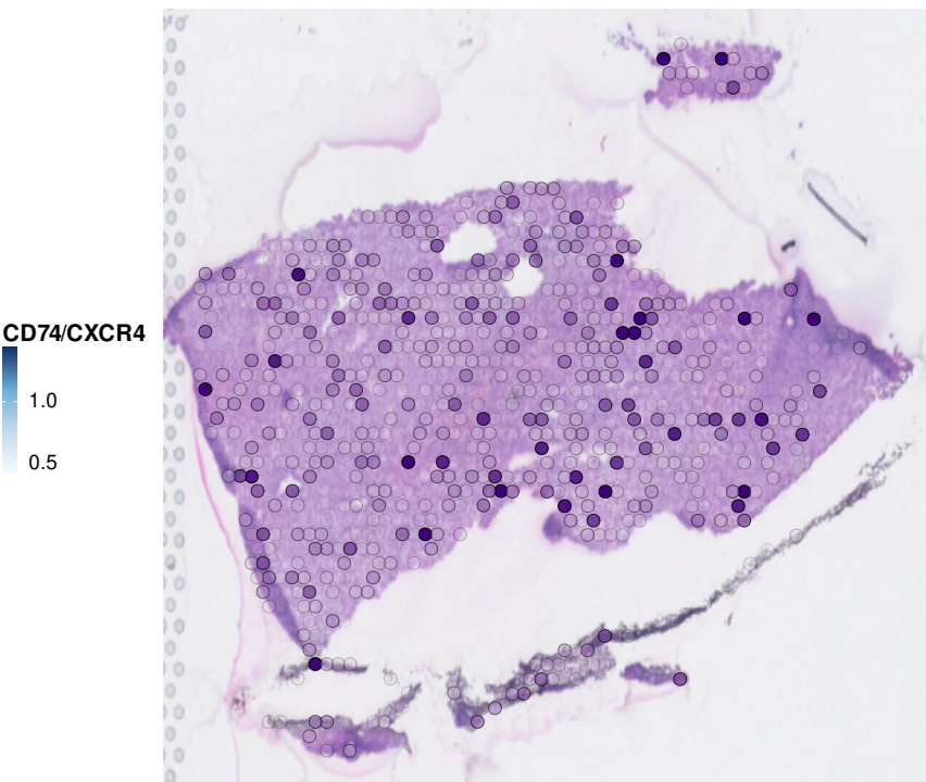
ECM-integrin context
