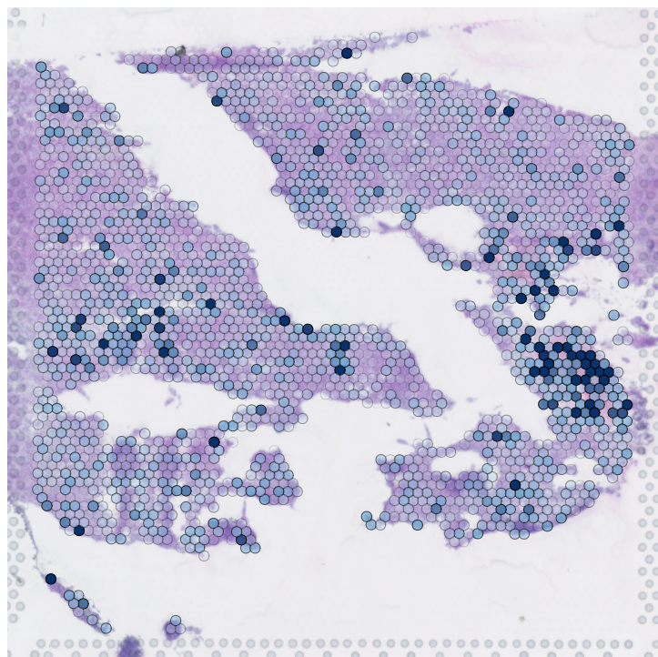
CD74/CXCR4
