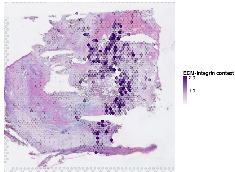
ECM-integrin context
