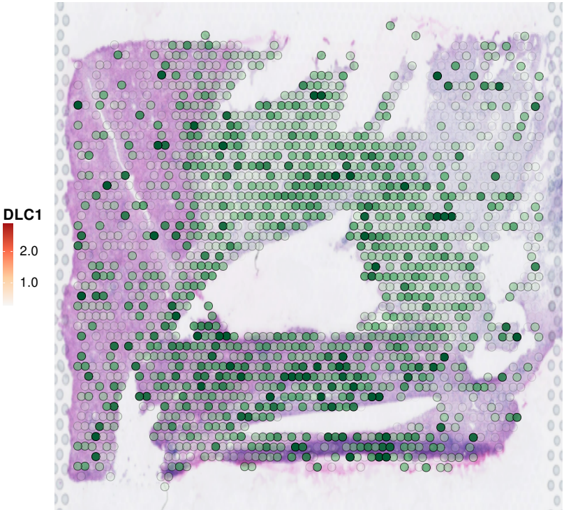
ECM-integrin context
