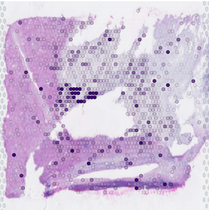
ECM-integrin context
