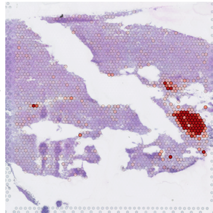
C3-like score
