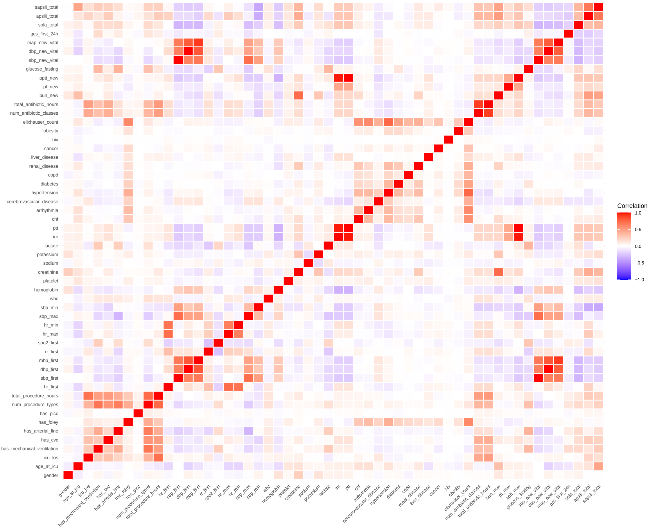
Spearman Correlation Matrix (Training Set)
