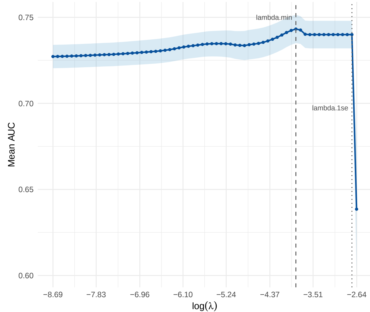
Cross-Validation Curve (AUC)
