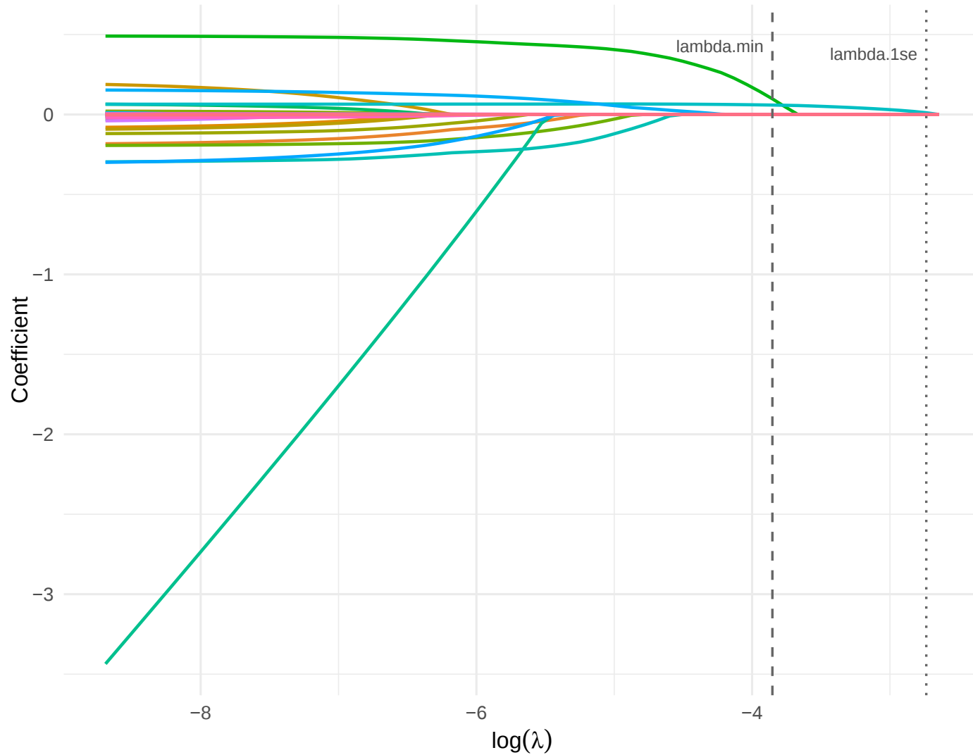
LASSO Coefficient Path
