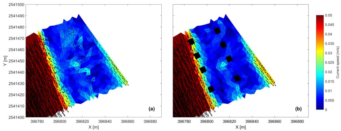
Figure S1. Surface current fields near the wharf under the 100-year flood condition: (a) no-pile case and (b) 8-square-pile case. The colour scale represents current speed, and the arrows indicate flow direction.
