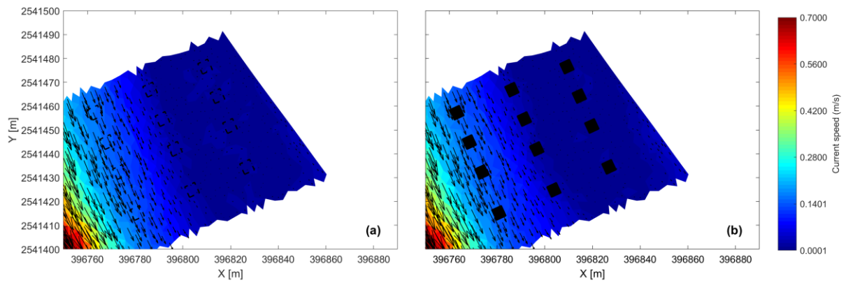
Figure S2. Surface current fields near the wharf under the 100-year flood condition: (a) no-pile case and (b) 12-square-pile case. The colour scale represents current speed, and the arrows indicate flow direction.
