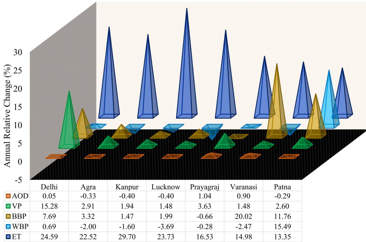
Figure 5: Annual relative changes (%) in landscape and atmospheric parameters within the 15 km RRZ of each study city (2015–2024)
