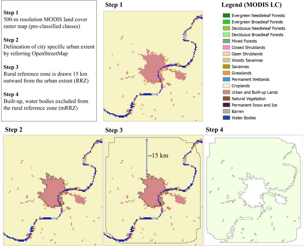
Figure 2: Methodological workflow for the delineation of urban extent, 15 km RRZ, mRRZ illustrated for Varanasi using the 2024 MODIS LULC product
