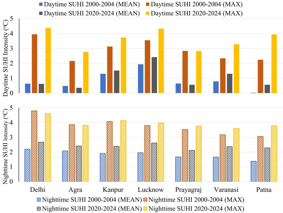
Figure 4: Comparison of mean and maximum SUHI intensities (°C) across the seven study cities for the 2000–2004 and 2020–2024 pentad windows; upper panel: daytime SUHI; lower panel: nighttime SUHI
