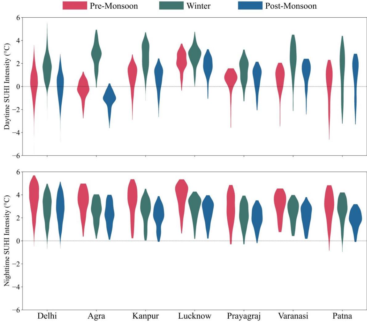
Figure 8: Pixel-level frequency distributions of seasonal daytime and nighttime SUHI intensities (°C) across the study cities (2020–2024)
