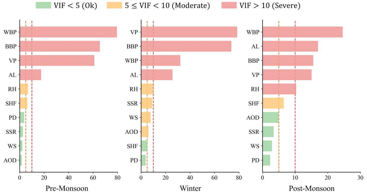
Figure 3: Seasonal multicollinearity checks for landscape and atmospheric predictors
