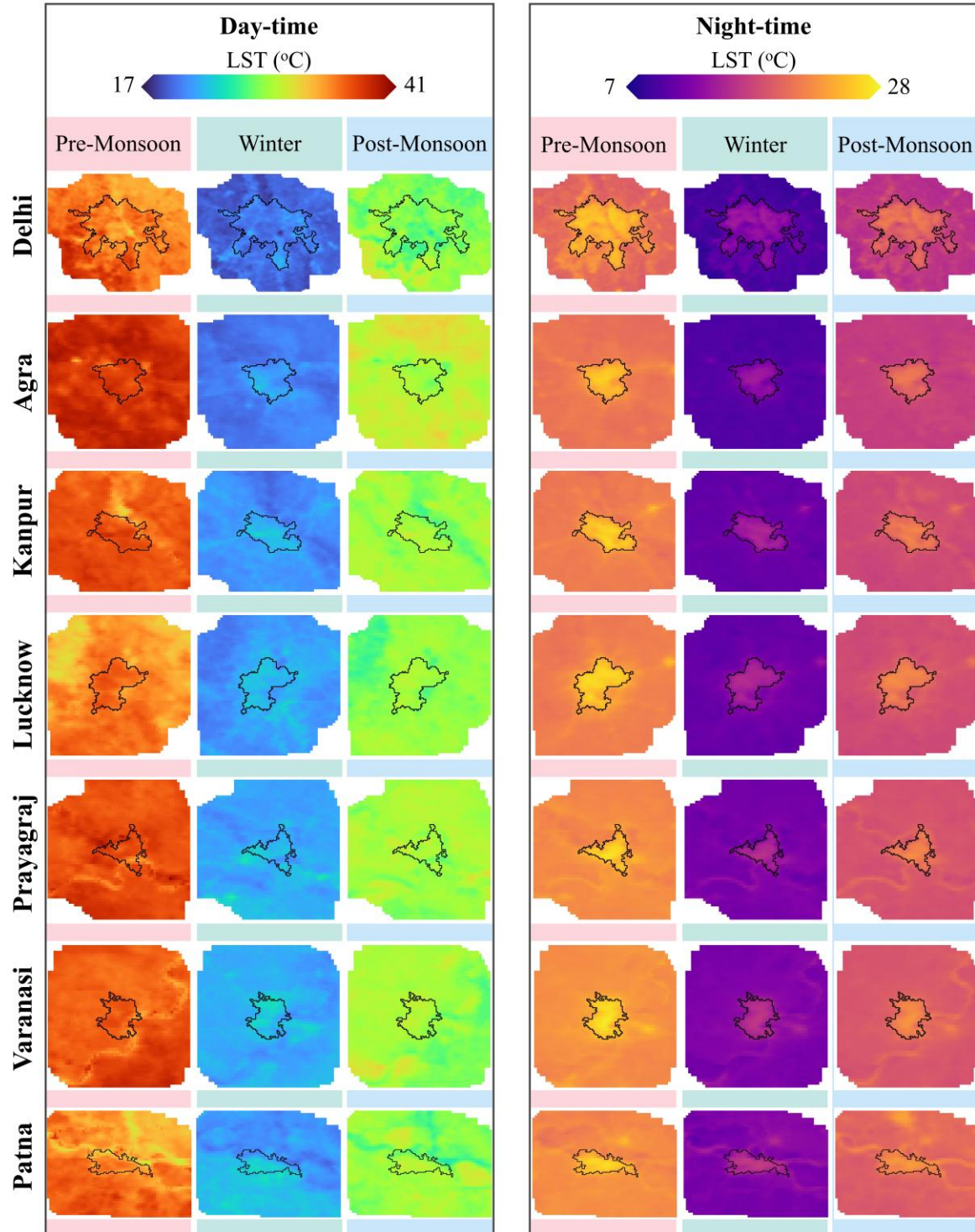
Figure 7: Spatial distribution of mean seasonal daytime and nighttime LST (°C) across the seven IGP cities and their 15 km RRZ during 2020–2024; black polygons denote the delineated urban boundaries
