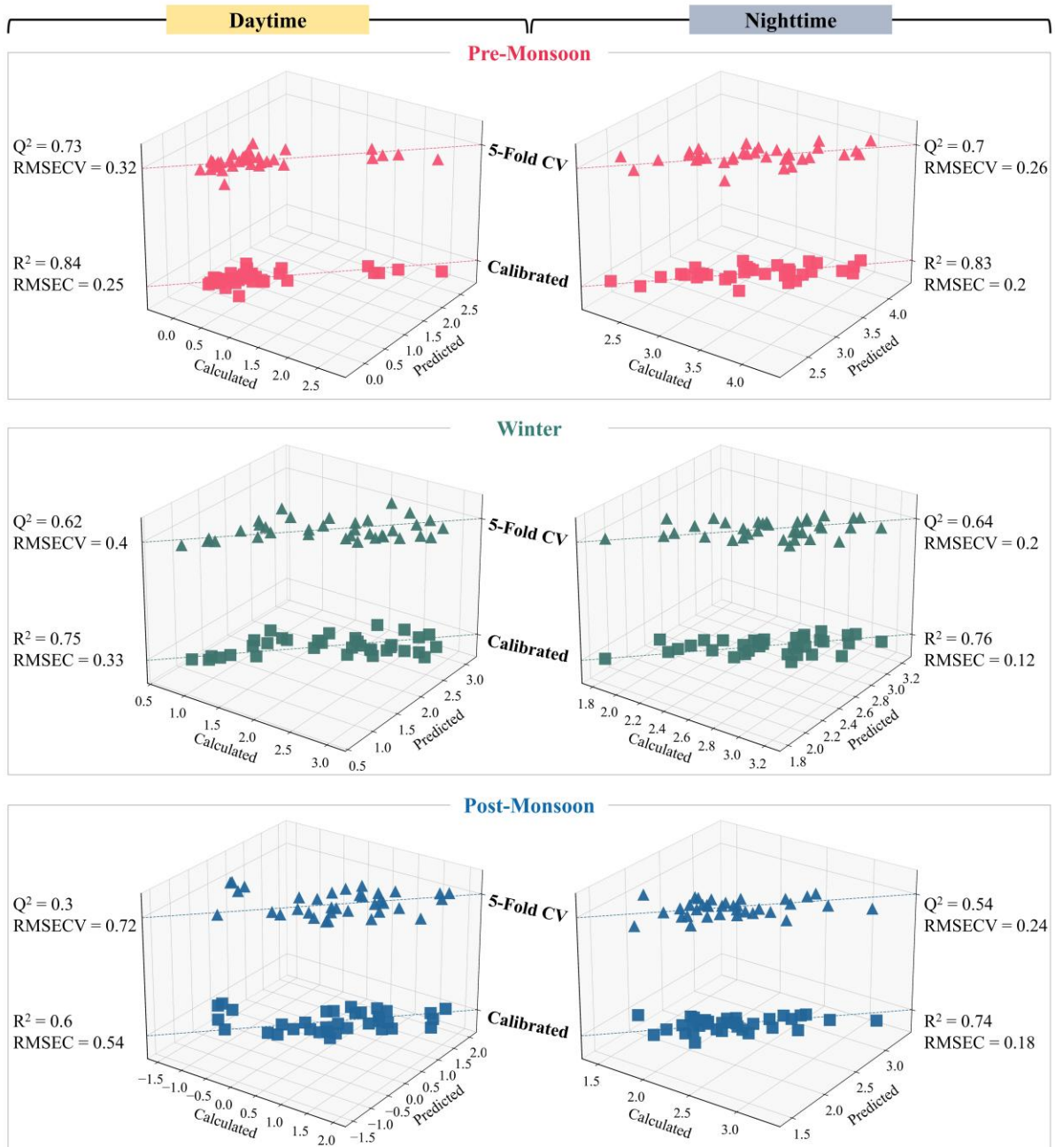
Figure 10: Diagnostic scatter plots of calibrated and 5-fold CV PLS regression models across seasonal regimes for daytime and nighttime
