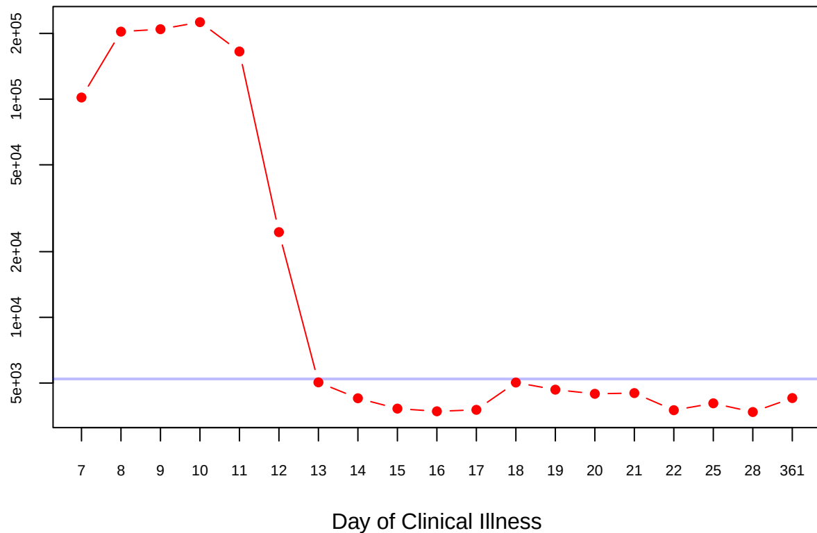
RB1 / Rb (5024-67)
