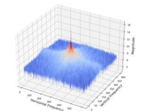
GT 3D Spectrum
