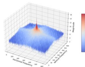
Ours 3D Spectrum
