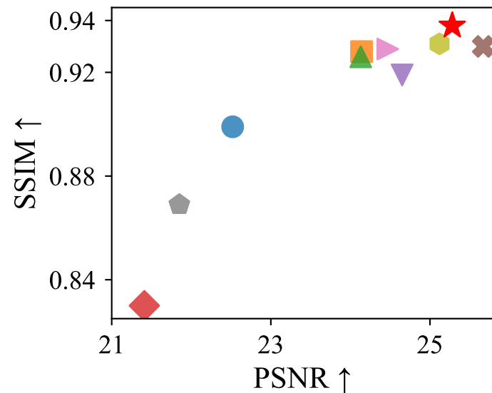
LOL-V2-Synthetic
