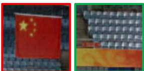
Retinexformer
