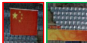
QuadPrior
