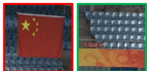
GT
