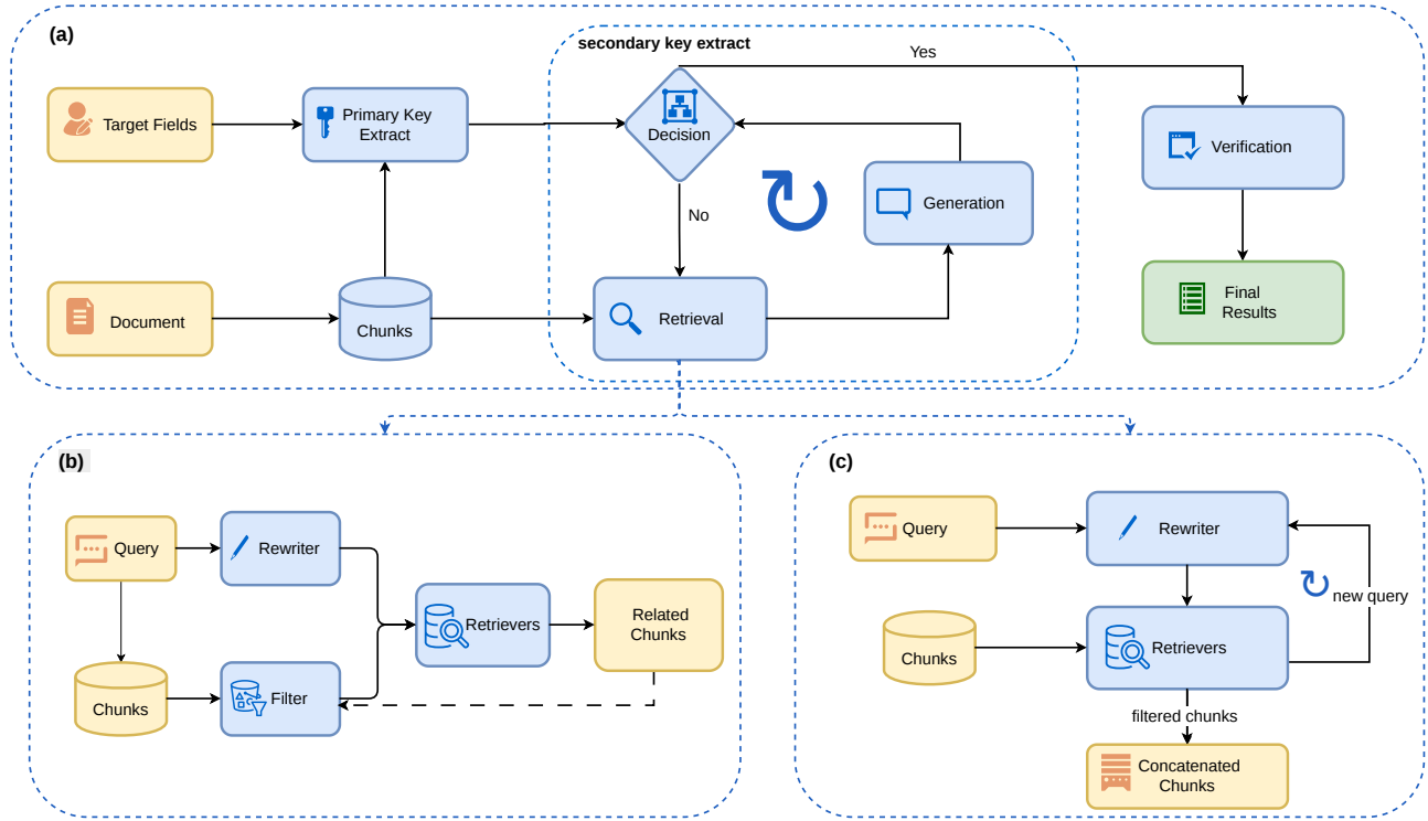
Figure 5. Architecture of the GeoExtractor framework. a , Overall modular agent architecture comprising six functional modules: document processing, primary key extraction, decision, retrieval, generation and validation. The decision module dynamically evaluates extraction completeness and controls iterative flow. b , Stage 1 retrieval: coverage-driven iterative retrieval with marked-chunk filtering to ensure non-redundant full-text coverage across iterations. c , Stage 2 retrieval: progressive multi-hop retrieval for complex fields requiring cross-paragraph reasoning, with LLM-driven query generation and important chunk extraction.
