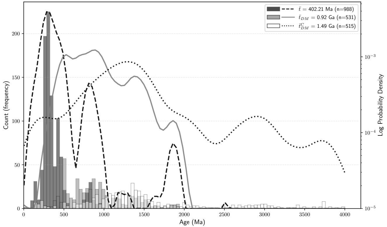
Figure 2. Histograms and probability density curves for the CAO magmatic rocks. a , Zircon U-Pb ages, showing a dominant peak at 500-300 Ma, a secondary peak at 1000-800 Ma, and sparse ages at 2000-1500 Ma. b , Zircon Hf model ages, exhibiting Precambrian tails extending to 3-4 Ga. c , Whole-rock Nd model ages, concentrated at 1.2-0.8 Ga with minimal Archean contributions.
