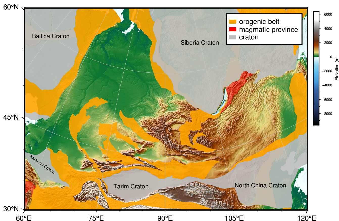
Figure 1. Tectonic map of CAOB, showing the distribution of major tectonic units, bounding cratons, and key suture zones. The CAOB extends from the Ural Mountains to the Pacific margin and is bounded by the East European, Siberian, Karakum, Tarim, and North China cratons. The orogen is composed of continental fragments, magmatic arcs, and subduction-accretion complexes. Topographic base map from NOAA National Geophysical Data Center.
