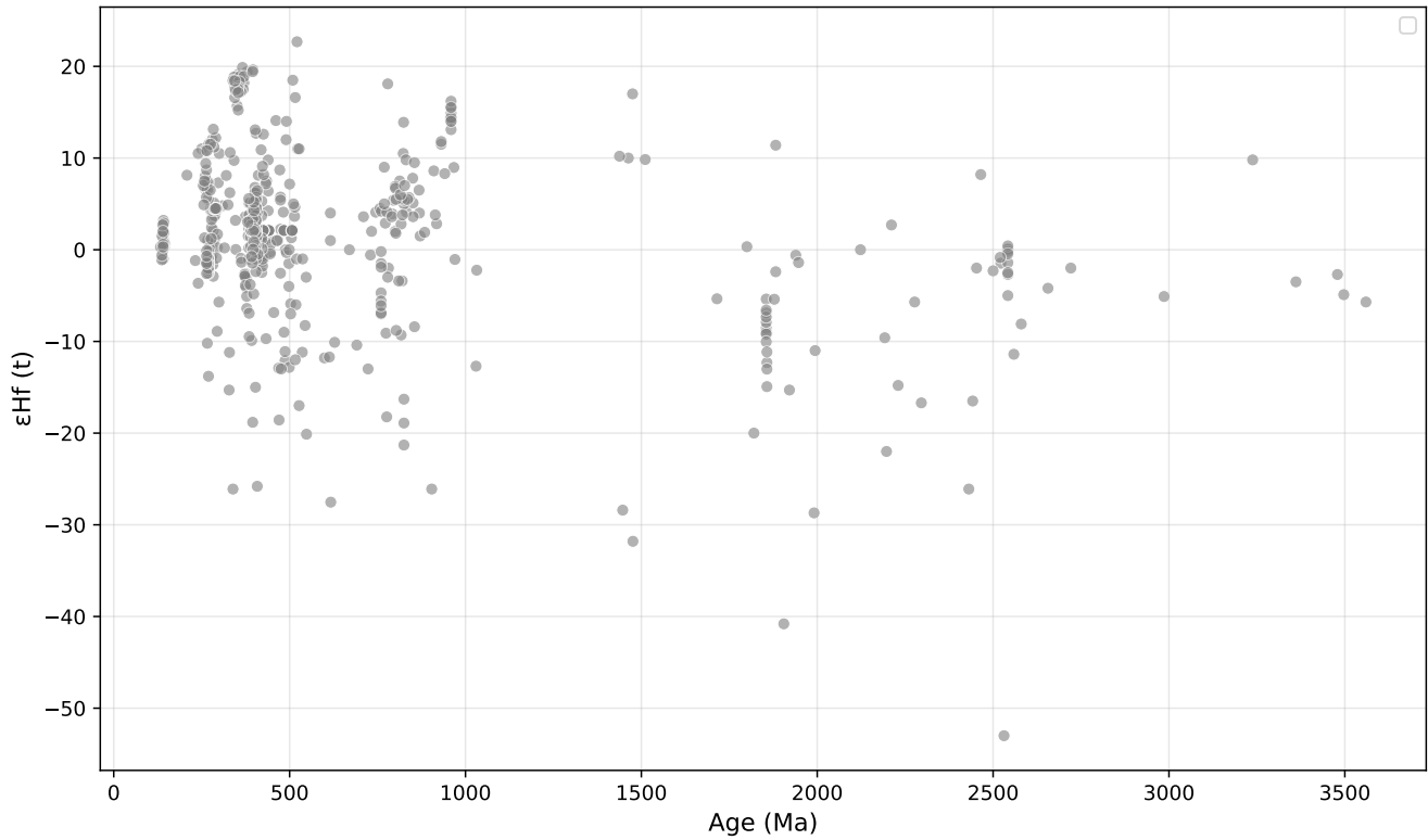
Figure 4. Zircon Hf-O isotopic data for CAOB magmatic rocks. a , \epsilon\text{Hf}(t) versus U-Pb age, showing three populations: highly positive (+10 to +20, 200-500 Ma), intermediate (0 to +10), and strongly negative (−10 to −50, 1500-3500 Ma). b , \delta^{18}\text{O} versus age, with values concentrated at 5.5-8.5‰ and a plateau at 400-500 Ma.
