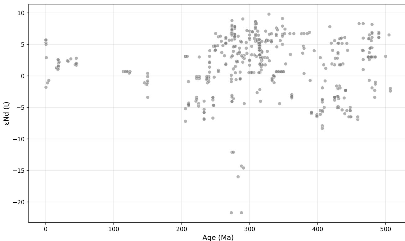
Figure 3. Sr-Nd isotopic data for igneous rocks from the Central Asian Orogenic Belt. a , \epsilon Nd(t) versus age, showing values spanning +8 to −22 with the majority clustering at +3 to +9. b , Initial ^{87}\text{Sr}/^{86}\text{Sr} versus age, concentrated at 0.703–0.707 with no systematic temporal trend.
