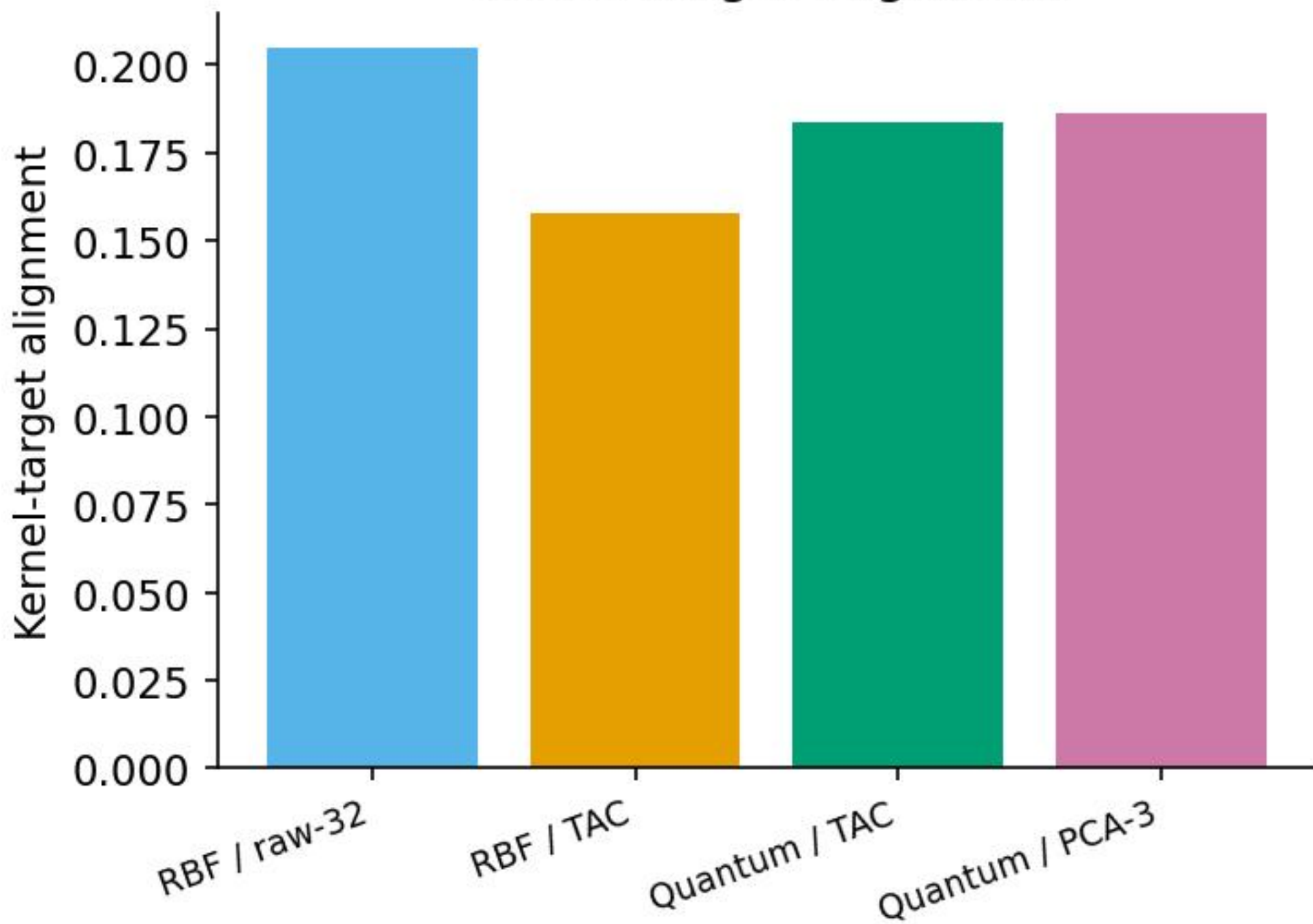
Kernel-target alignment
