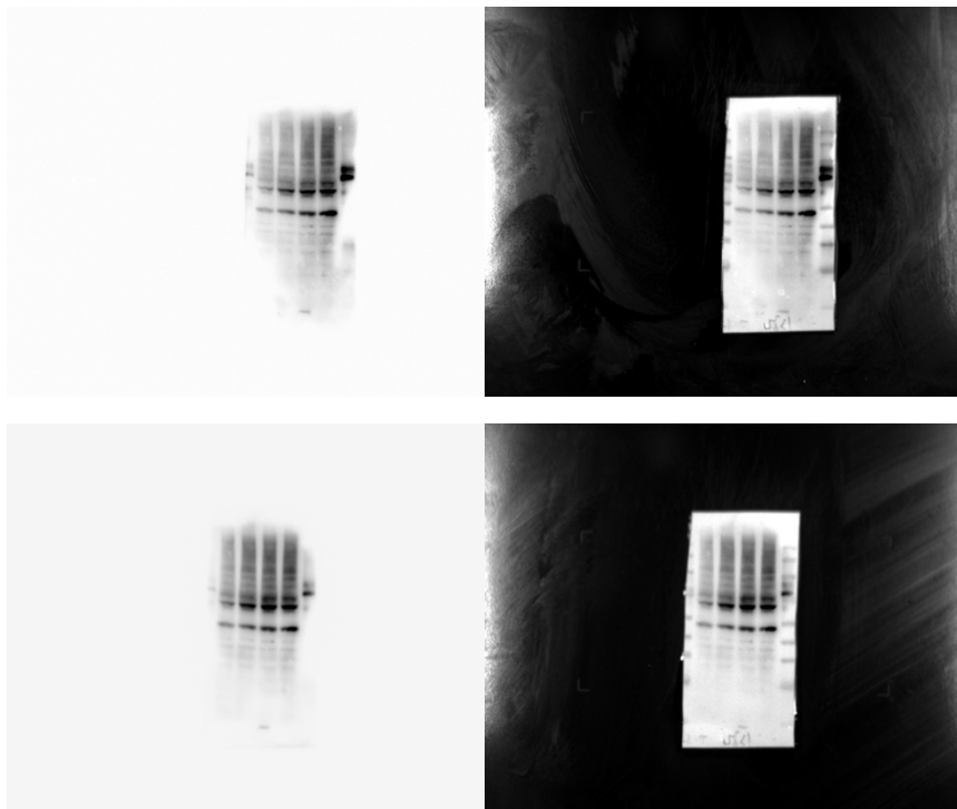
Figure6A_T47D_HSP90_overexpression_HSP90_betaActin_uncropped_whole_blot.tif
