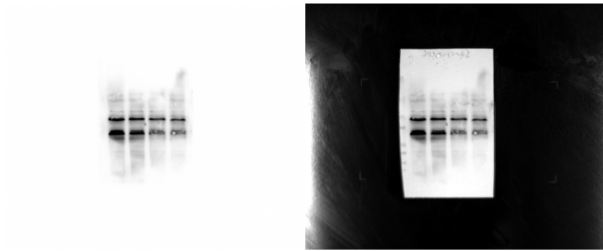
Figure6A_T47D_HSP90_knockdown_HSP90_betaActin_uncropped_whole_blot.tif
