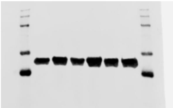
Actin
