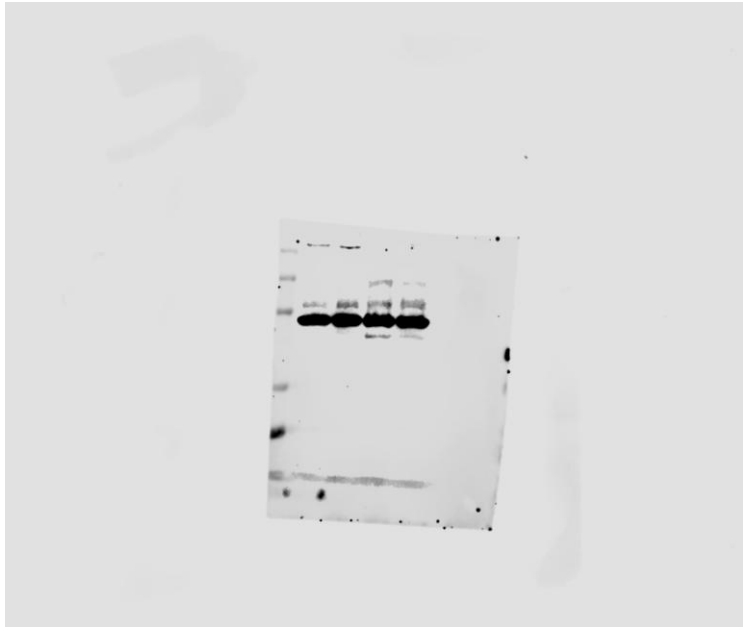
Actin
