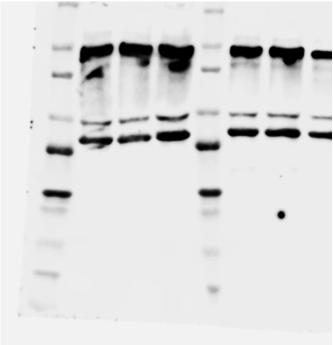
Actin
