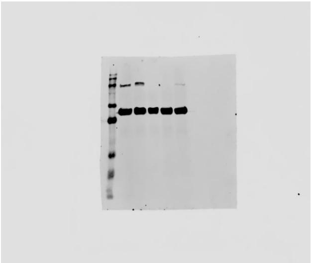
Actin
