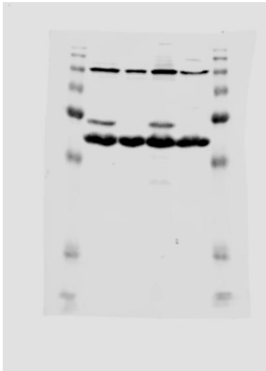
Actin
