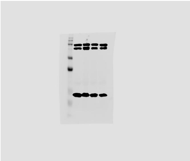
Actin
