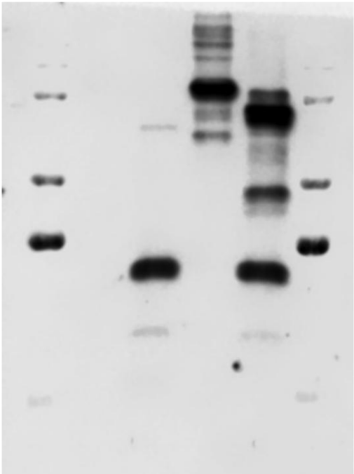
Calpain -1
