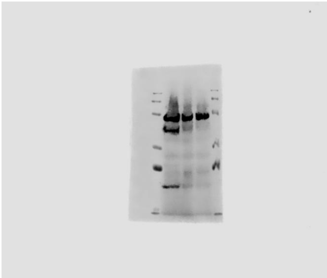
Calpain-1
