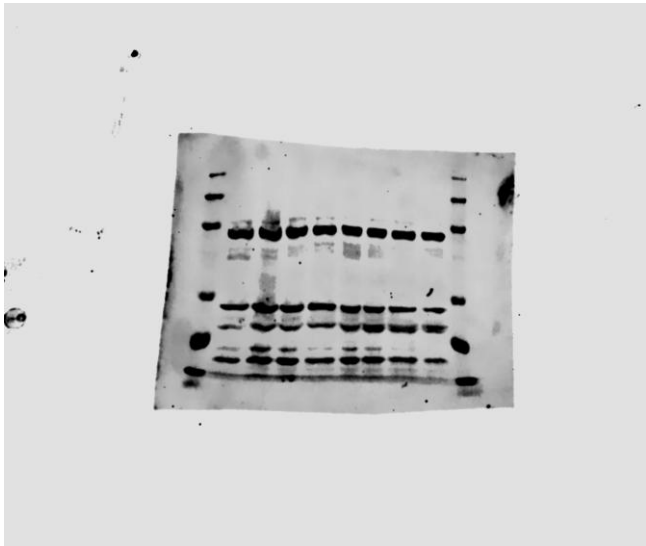
Actin
