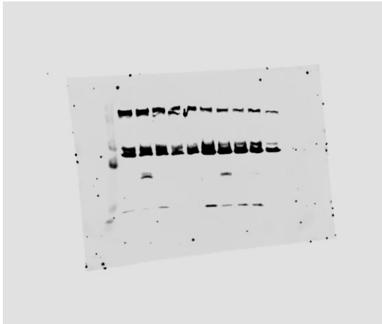
ACTIN
