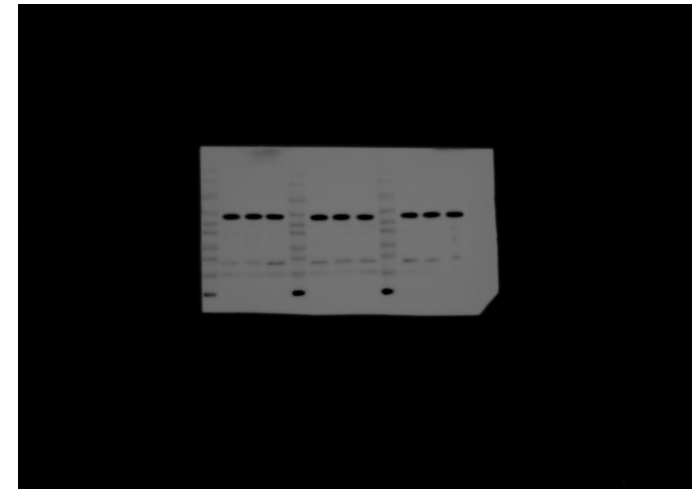
\beta -actin
