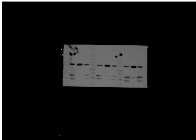
SOX2
