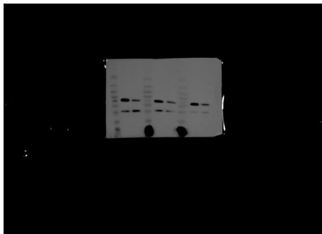
SOX2
