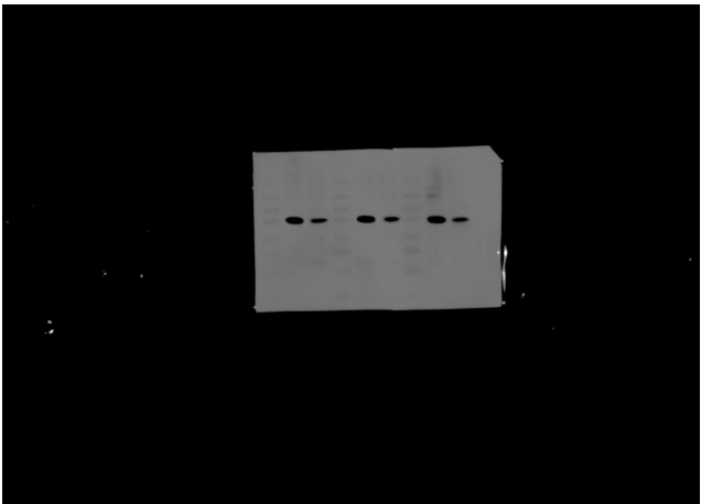
SOX2
