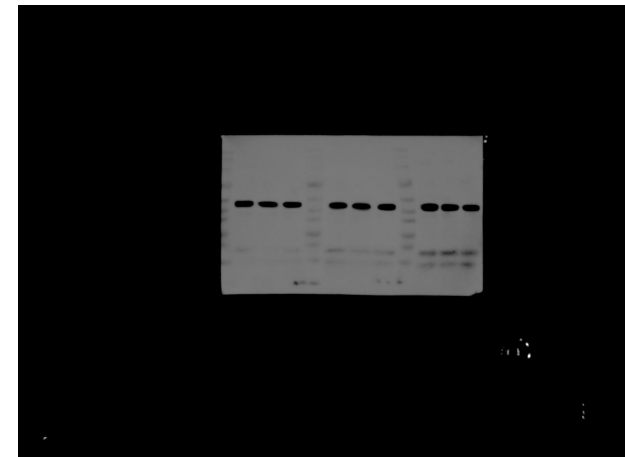
β-actin
