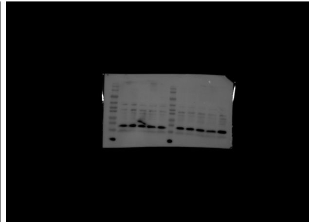
COXIV
