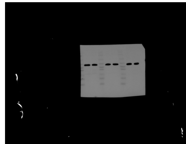
β-actin
