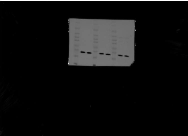
COXIV
