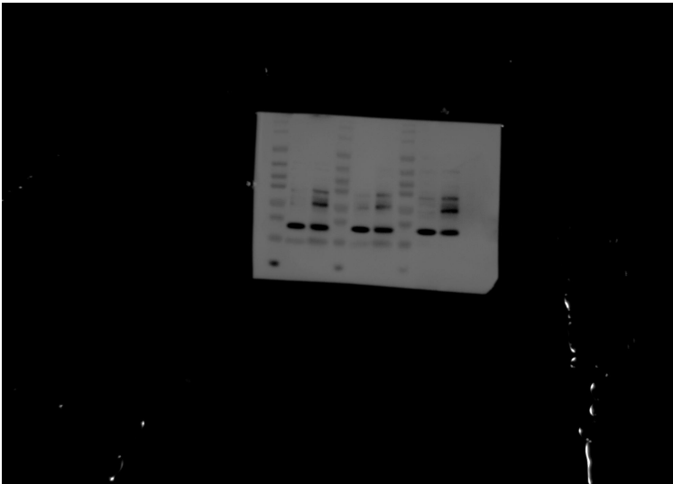
COXIV
