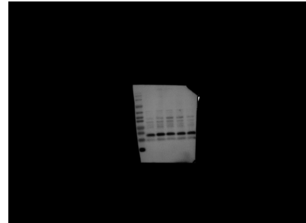
COXIV
