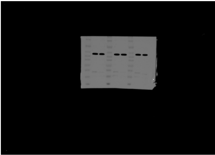
β-actin
