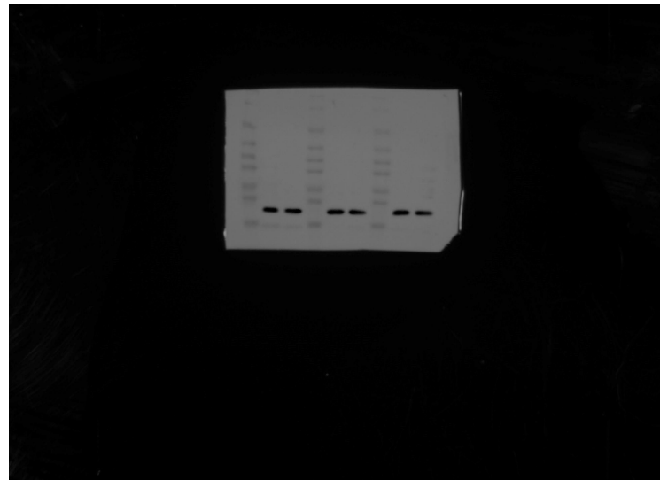
COXIV
