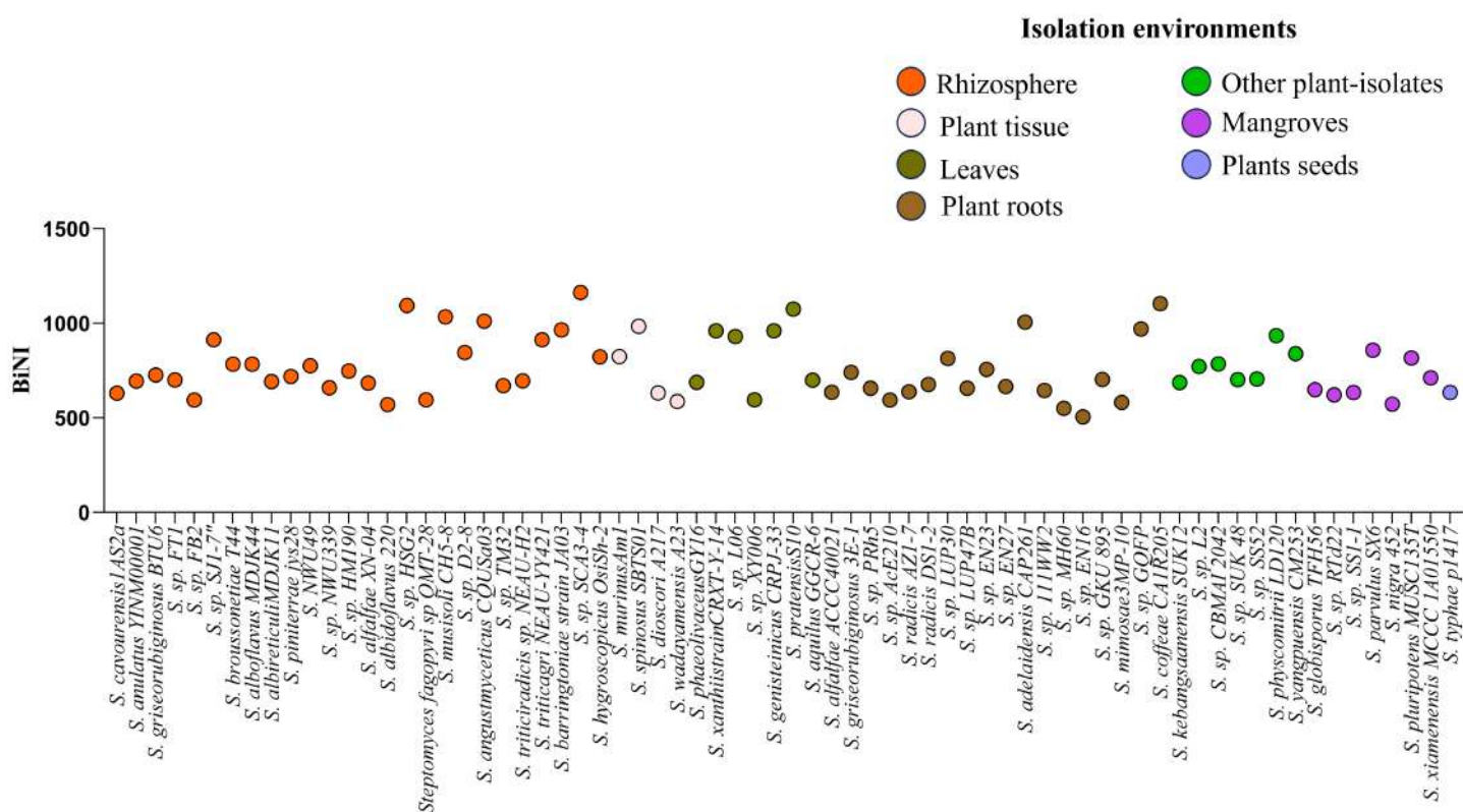
Supplementary Figure 4. Biosynthetic novelty index (BiNI) of Rhizosphere and another plant-associated Streptomyces .
