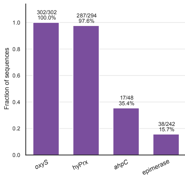
Figure S1. De novo motif analysis. Bars show the fraction of sequences in analyzed groups that contained a de novo motif matching either the E. coli or P. aeruginosa OxyR PWM. Bar labels give positive sequences over total sequences in analyzed groups, followed by the percentage.
